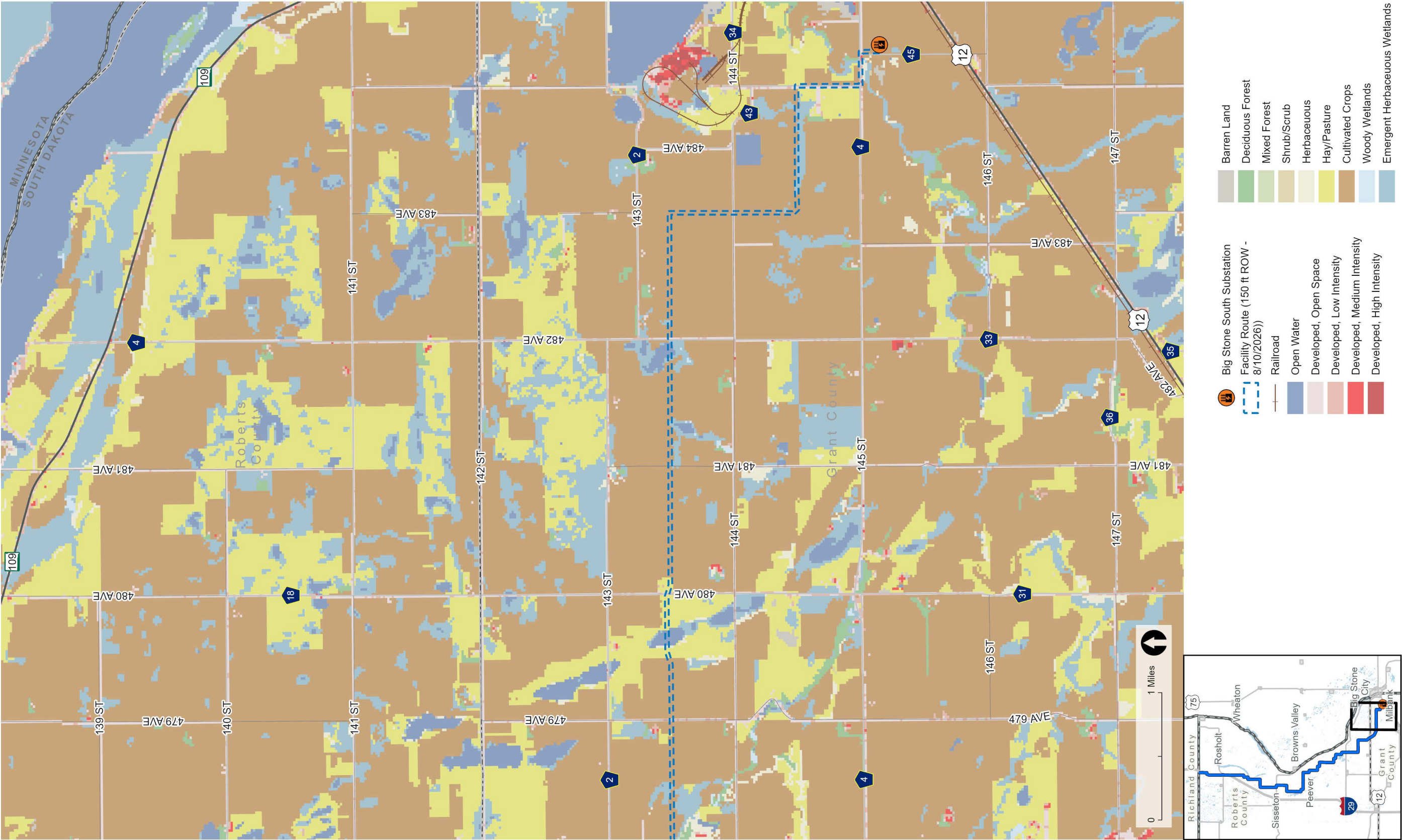
Figure 11 Land Cover
