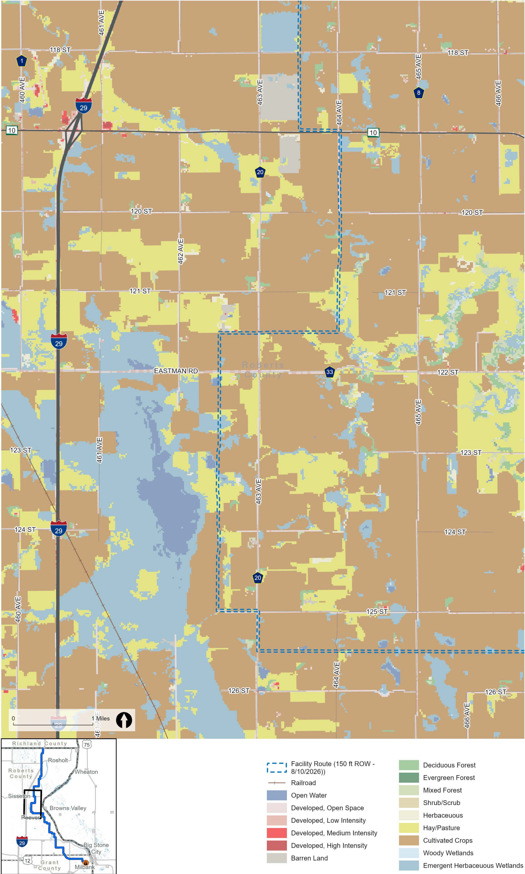
Figure 11 Land Cover
