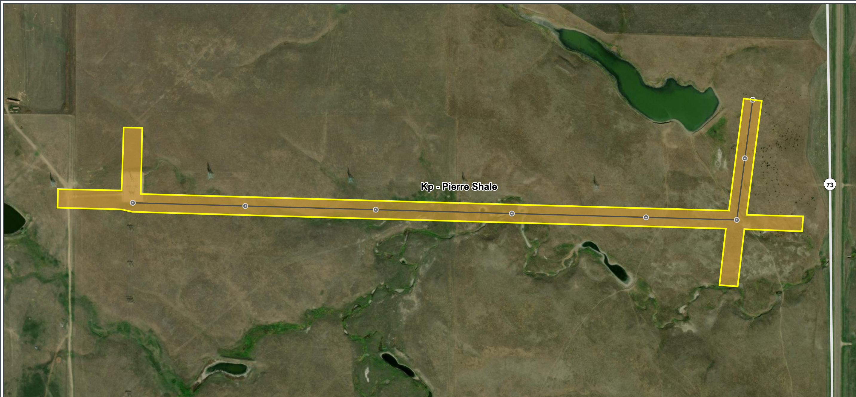
Figure A-5 Bedrock Geology Map Haakon Co, South Dakota
