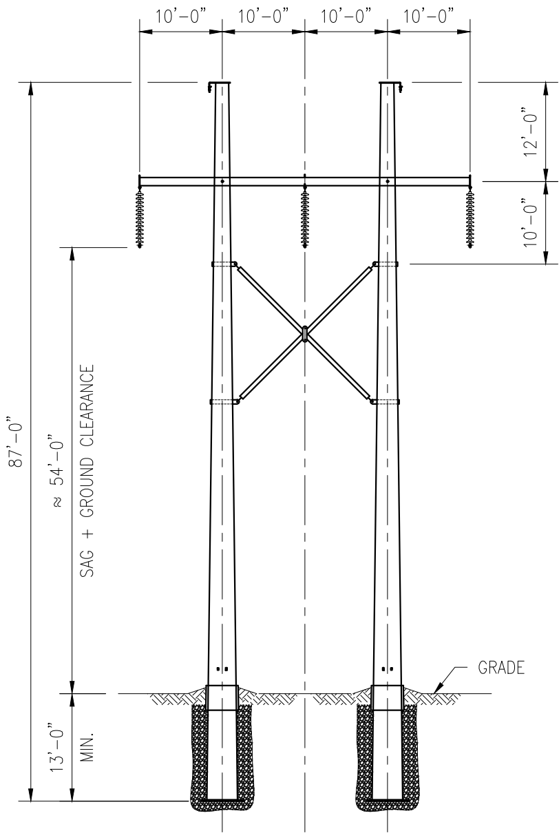
230KV TYPE 2HS SINGLE CIRCUIT H-FRAME TANGENT STRUCTURE AVERAGE SPAN \approx 800'
