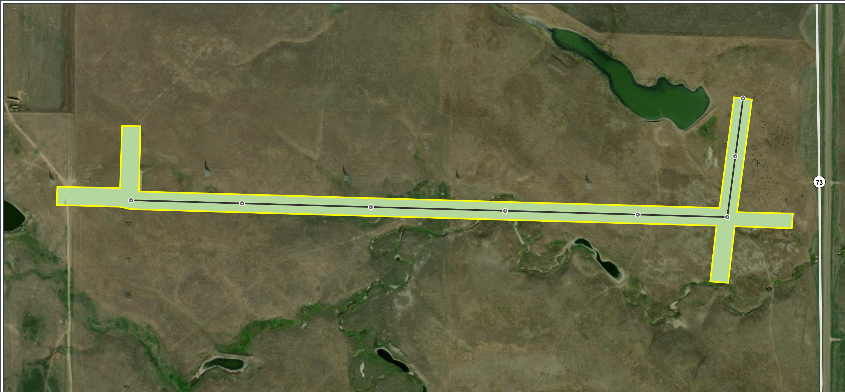
Figure A-10 NLCD Map Haakon Co, South Dakota
