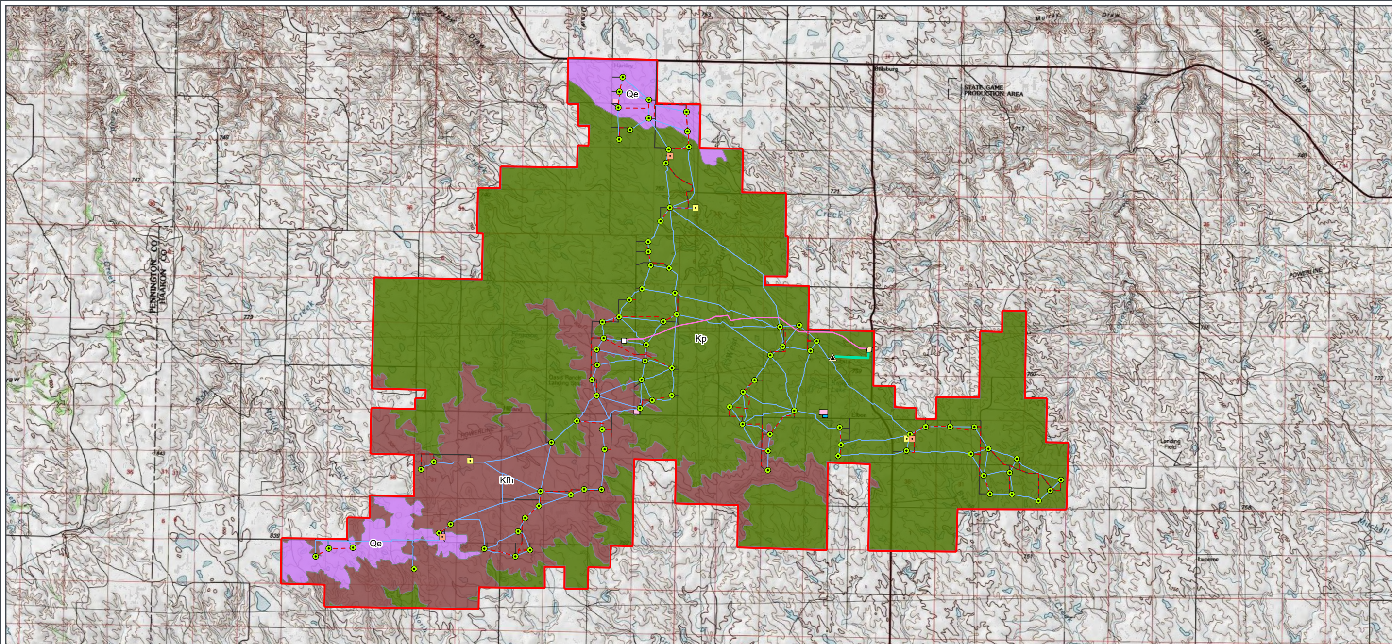
Figure A-6 Bedrock Geology Map Philip Wind Project Haakon Co, South Dakota
