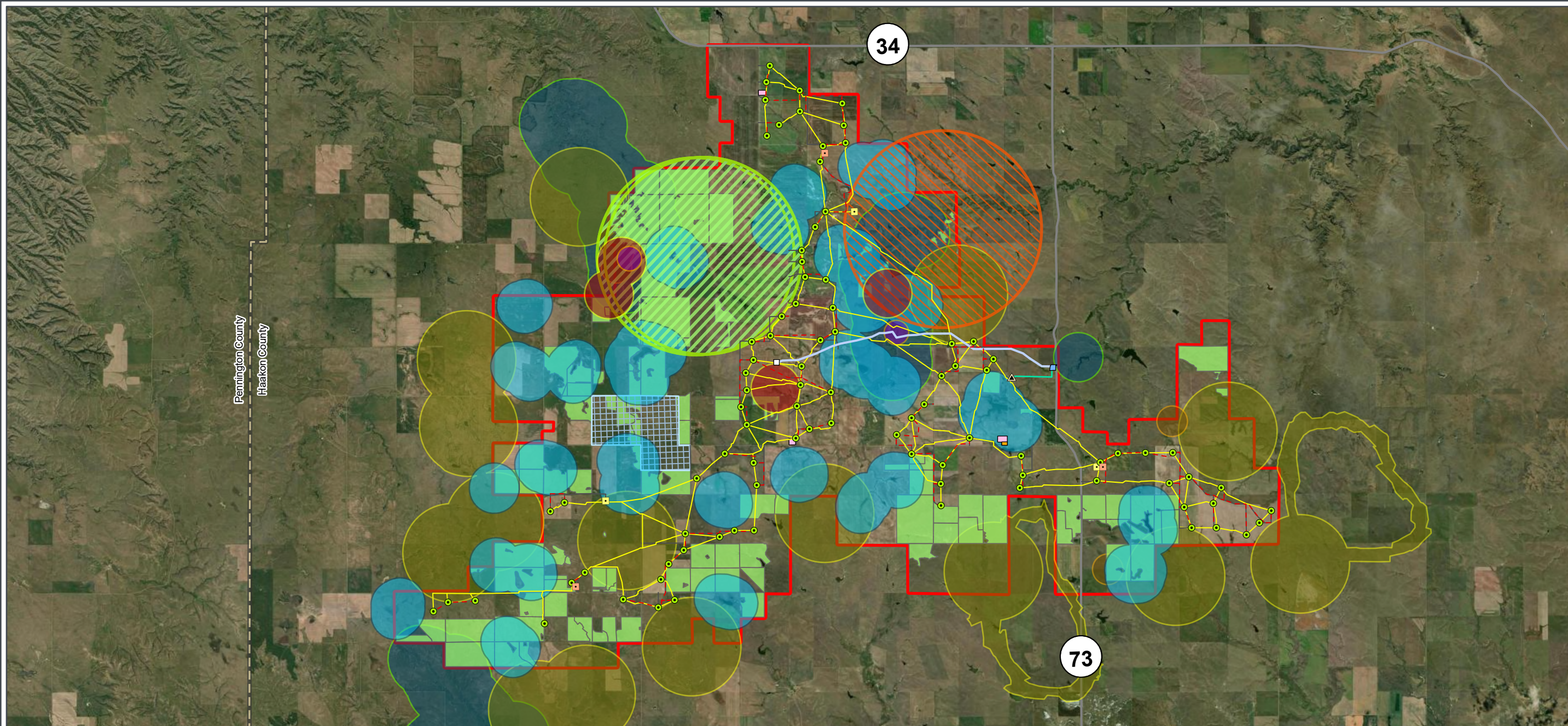
Figure A-4 Siting Constraints Map Philip Wind Project Haakon Co, South Dakota
