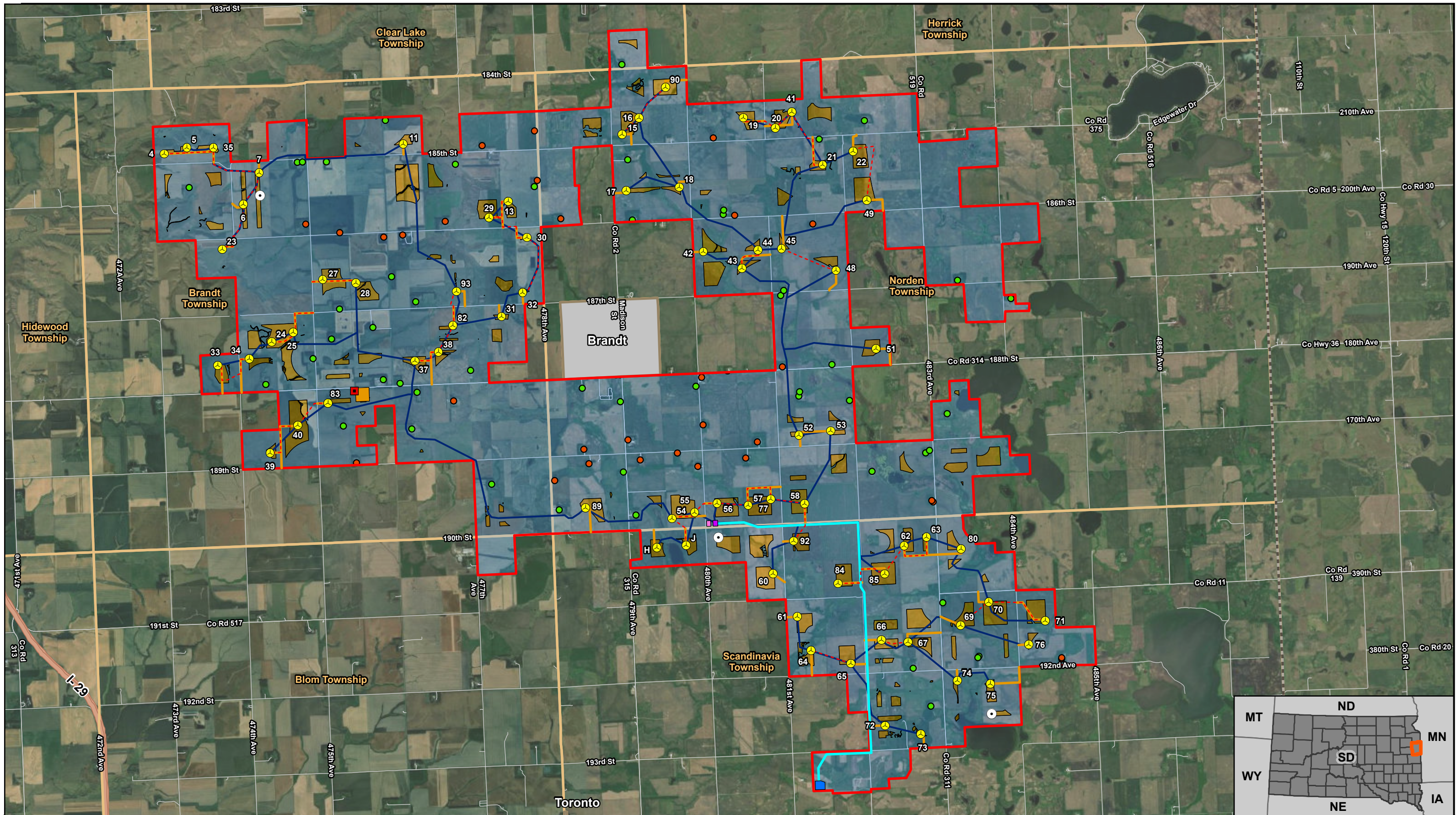
Figure 4 Turbine Siting Constraints Map South Deuel Wind Project Deuel County, South Dakota
