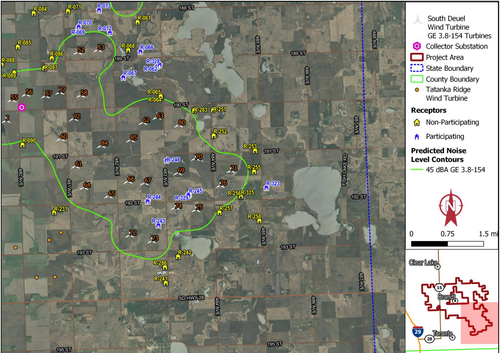
Figure D-8. Noise Level Contours – GE 3.8-154 Turbines - Southeast Area
