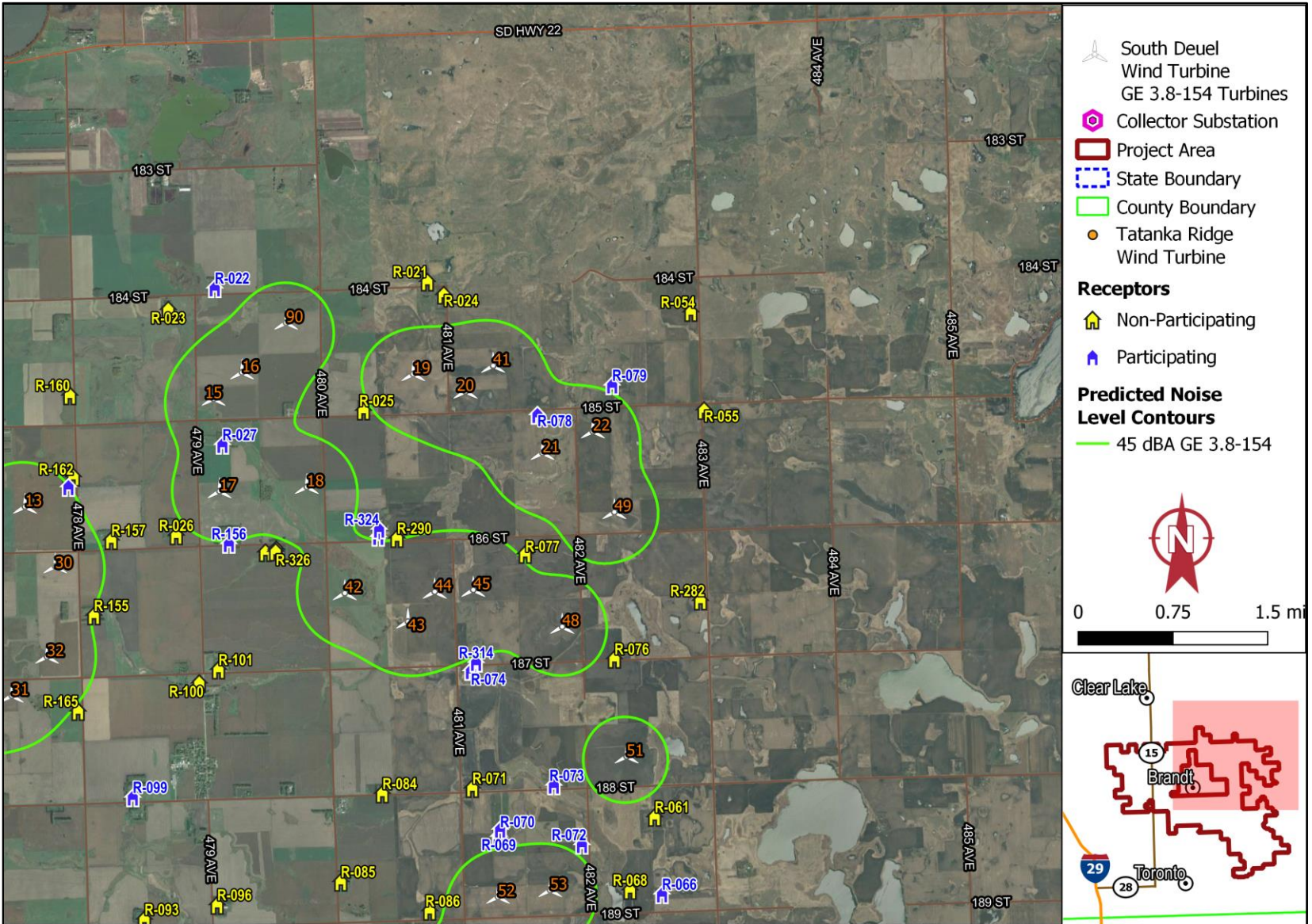
Figure D-6. Noise Level Contours – GE 3.8-154 Turbines - Northeast Area
