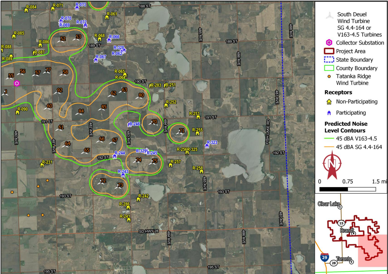
Figure D-4. Noise Level Contours – SG 4.4-164 and V163-4.5 Turbines - Southeast Area
