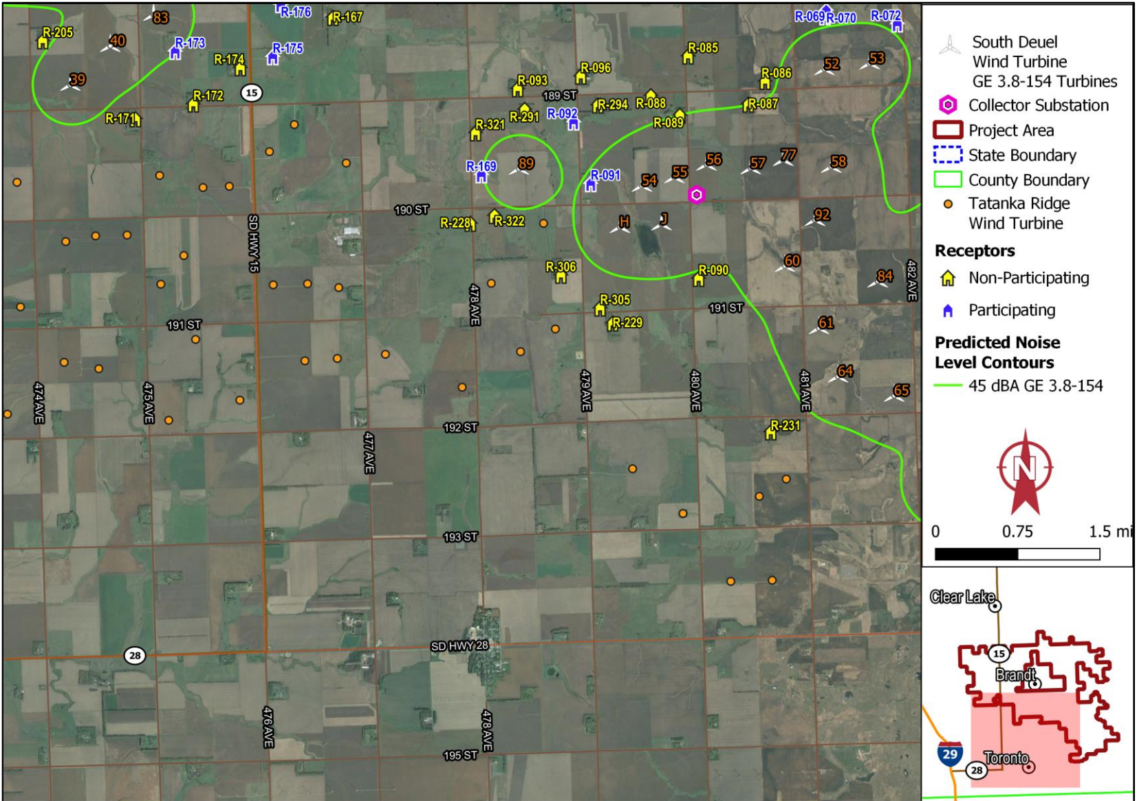
Figure D-7. Noise Level Contours – GE 3.8-154 Turbines - Southwest Area
