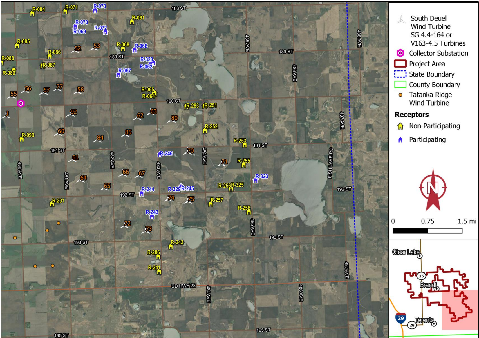
Figure A-4. Modeled Locations – SG 4.4-164 or V163-4.5 Turbines - Southeast Area
