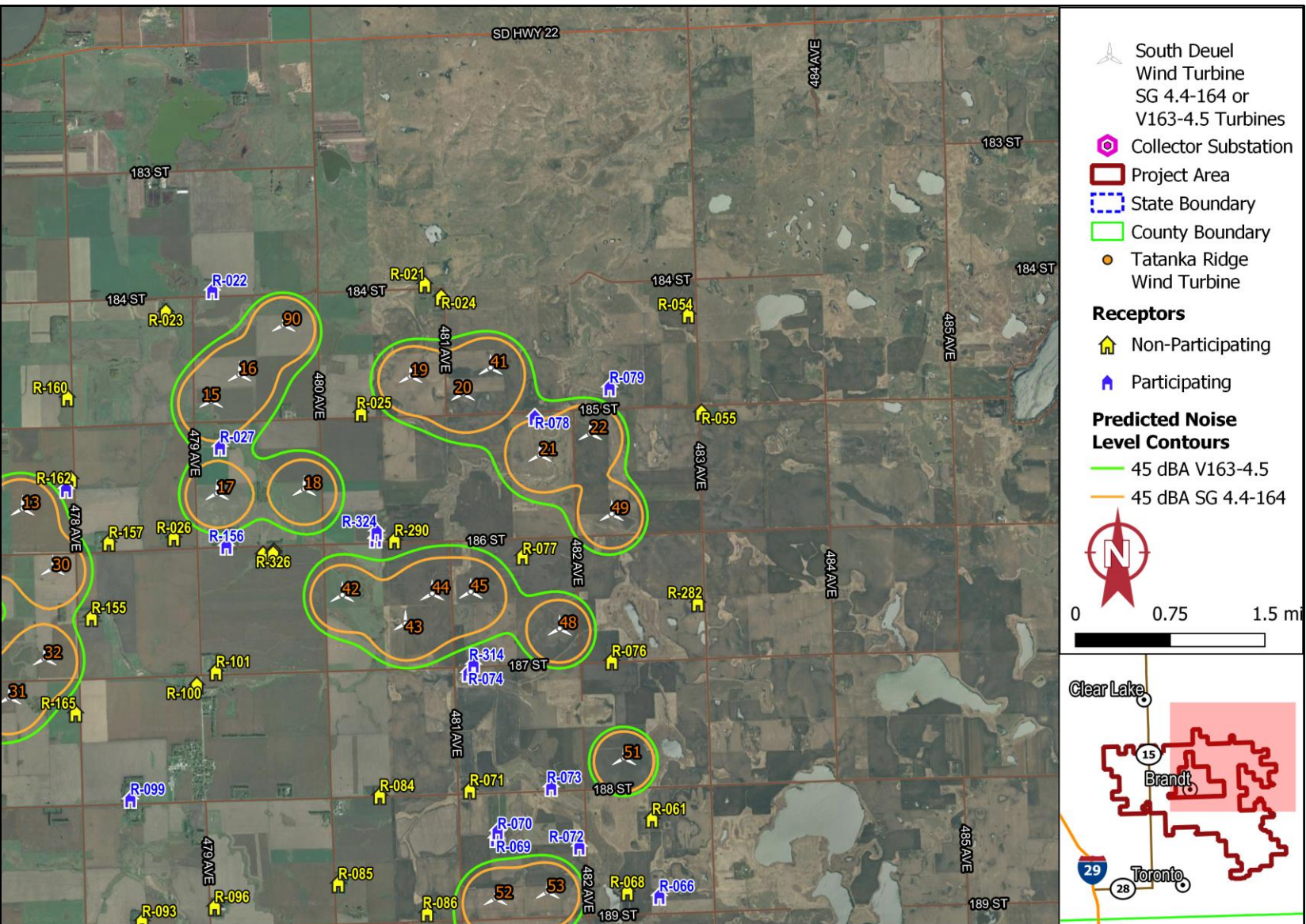
Figure D-2. Noise Level Contours – SG 4.4-164 and V163-4.5 Turbines - Northeast Area
