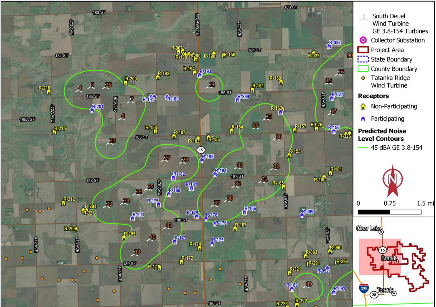
Figure D-5. Noise Level Contours – GE 3.8-154 Turbines - Northwest Area
