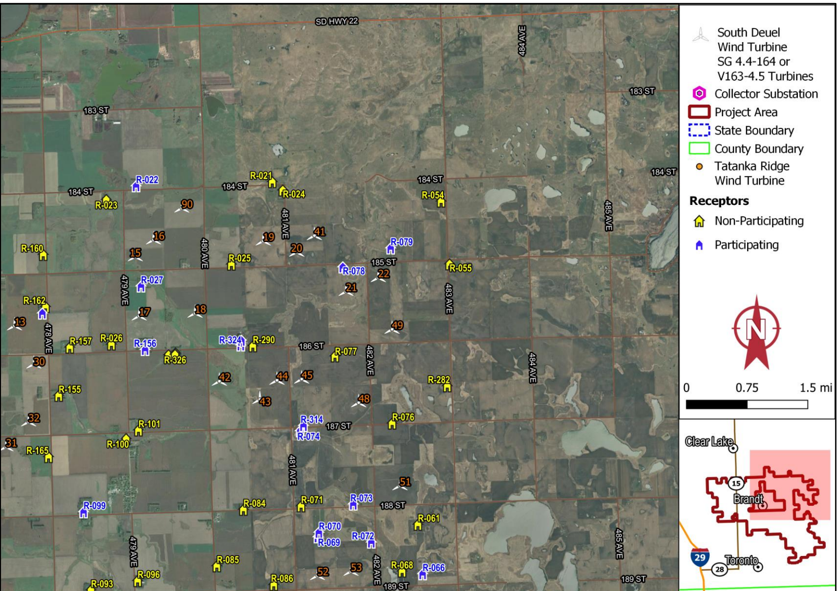
Figure A-2. Modeled Locations – SG 4.4-164 or V163-4.5 Turbines - Northeast Area
