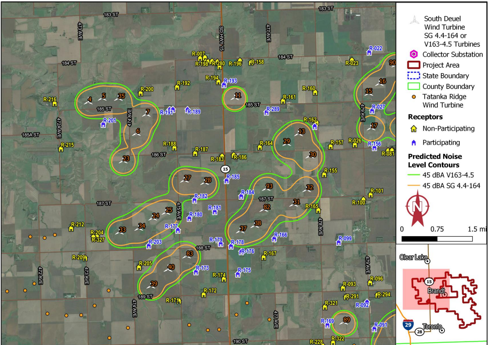
Figure D-1. Noise Level Contours – SG 4.4-164 and V163-4.5 Turbines - Northwest Area
