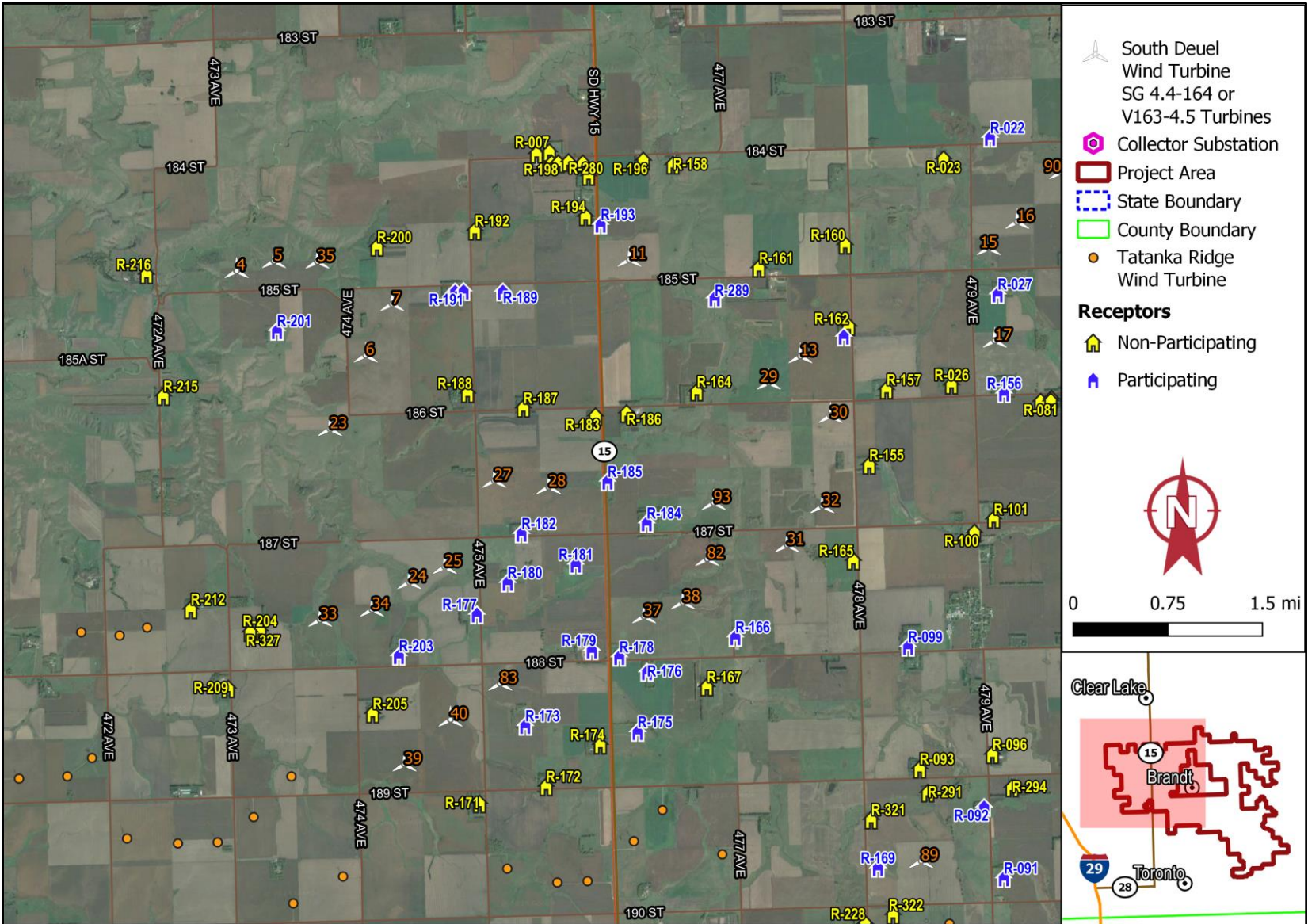
Figure A-1. Modeled Locations – SG 4.4-164 or V163-4.5 Turbines - Northwest Area
