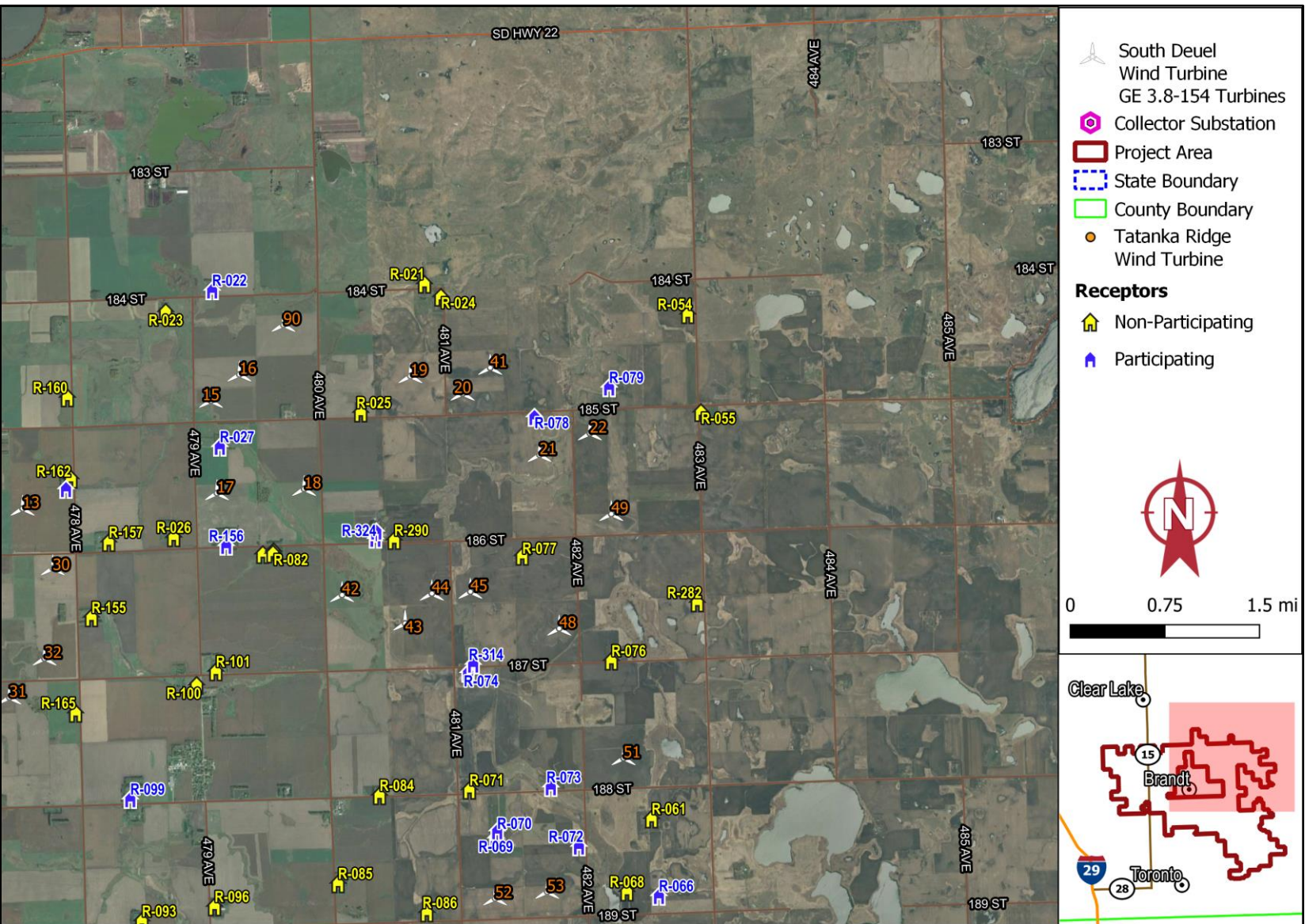
Figure A-6. Modeled Locations – GE 3.8-154 Turbines - Northeast Area
