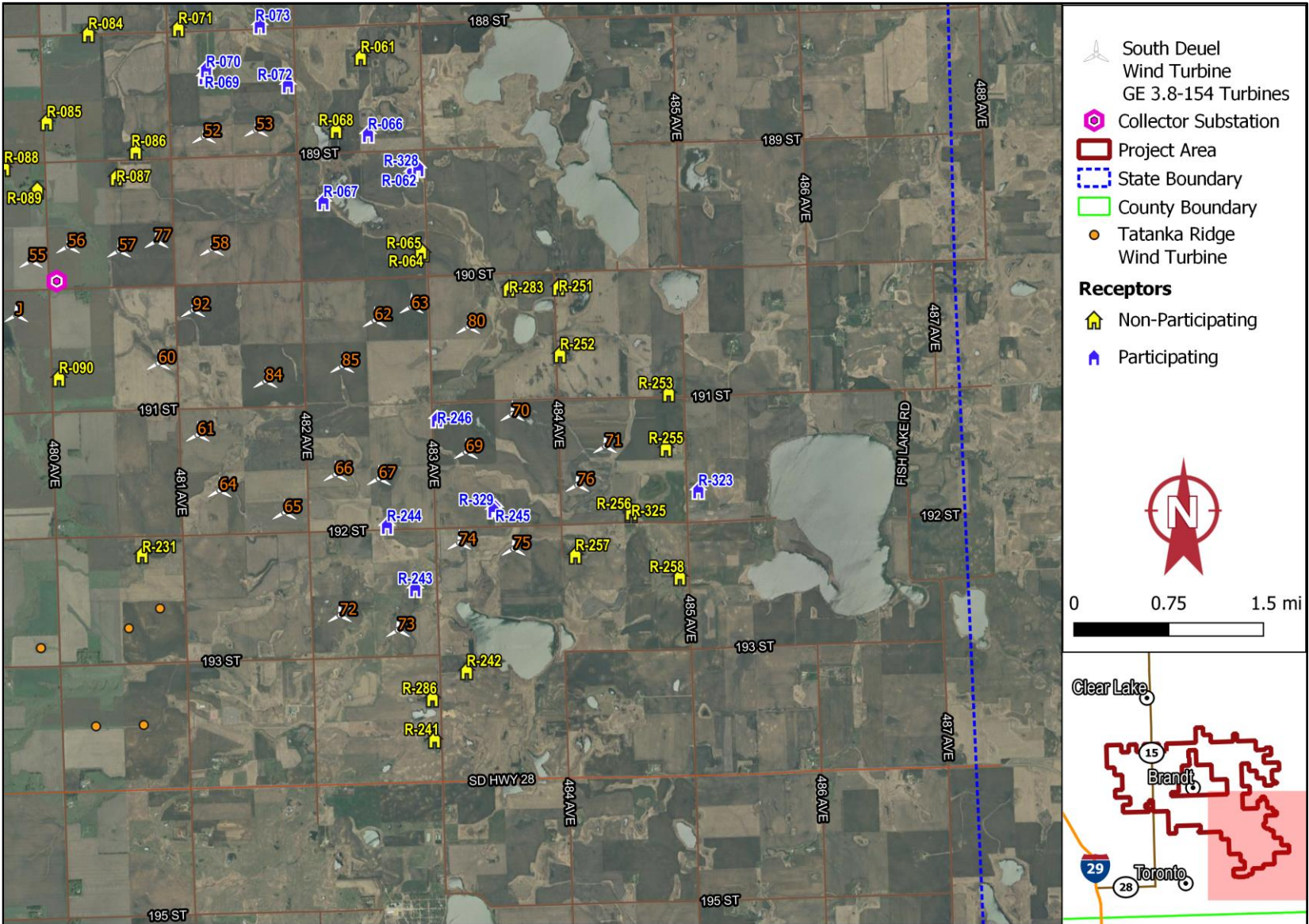
Figure A-8. Modeled Locations – GE 3.8-154 Turbines - Southeast Area
