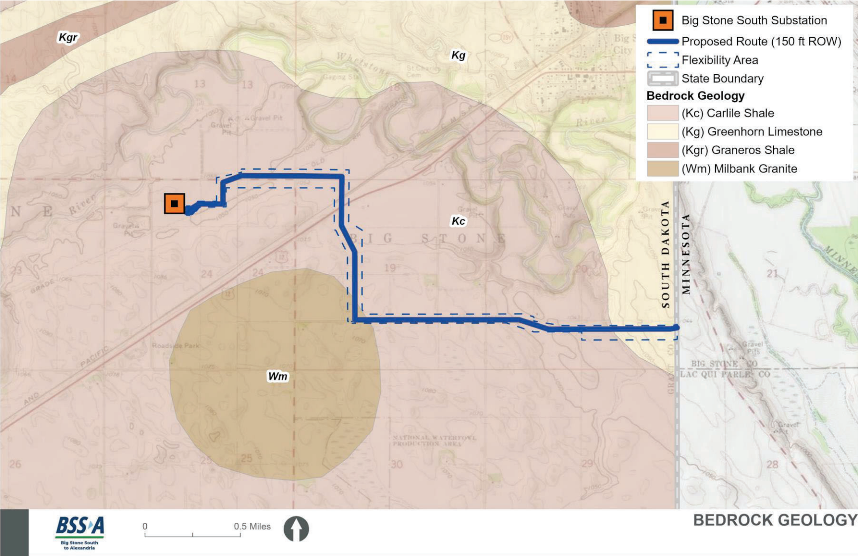
Figure 8. Bedrock geology
