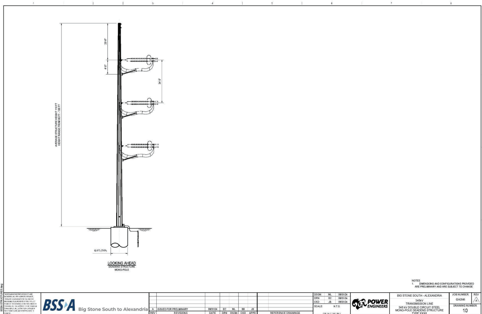
Figure 5. Example 345 kV double circuit steel monopole deadend structure configuration
