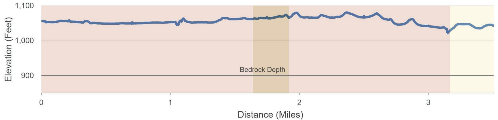
Bedrock Geology Cross Section
