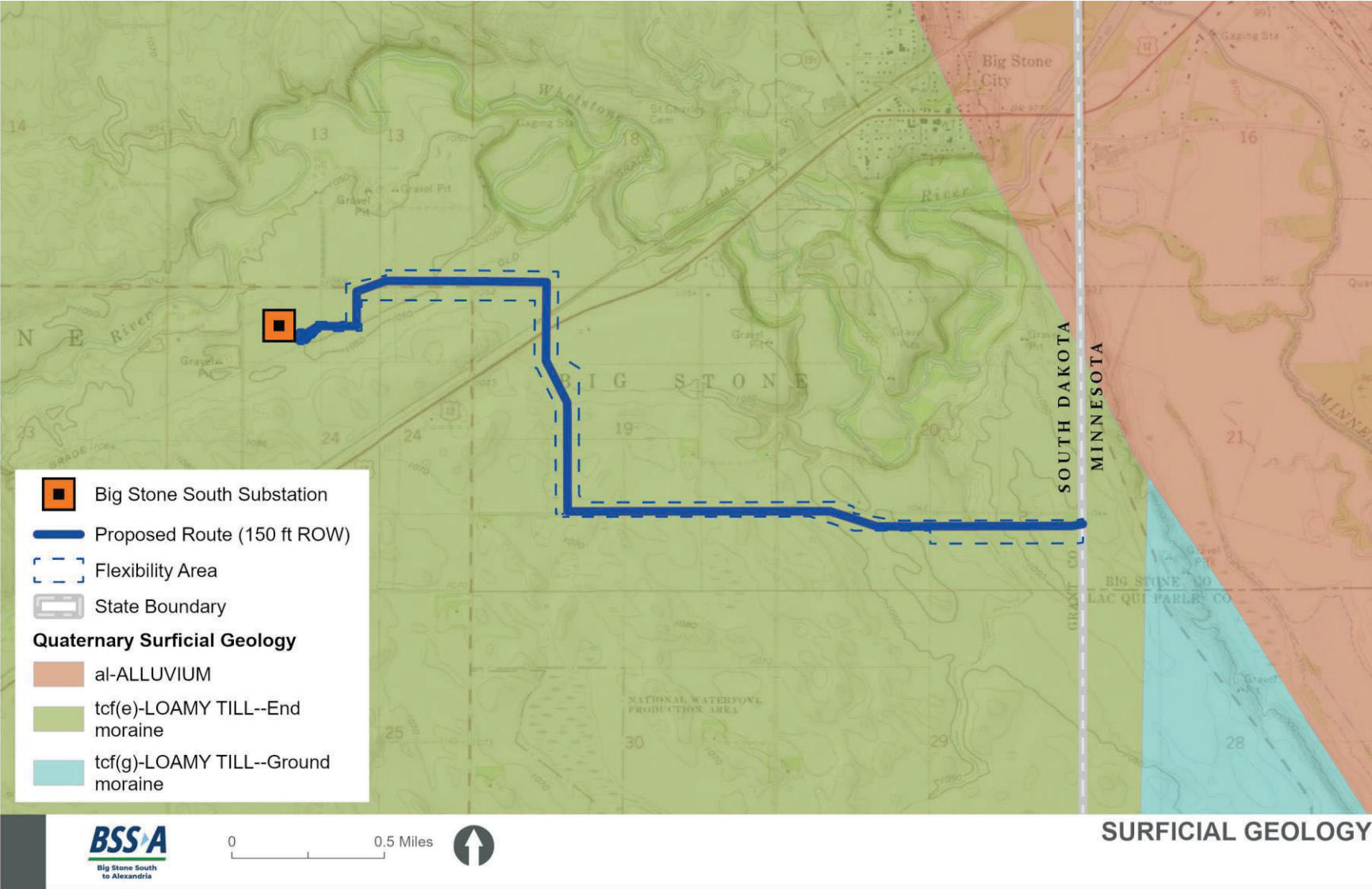
Figure 9. Surficial geology
