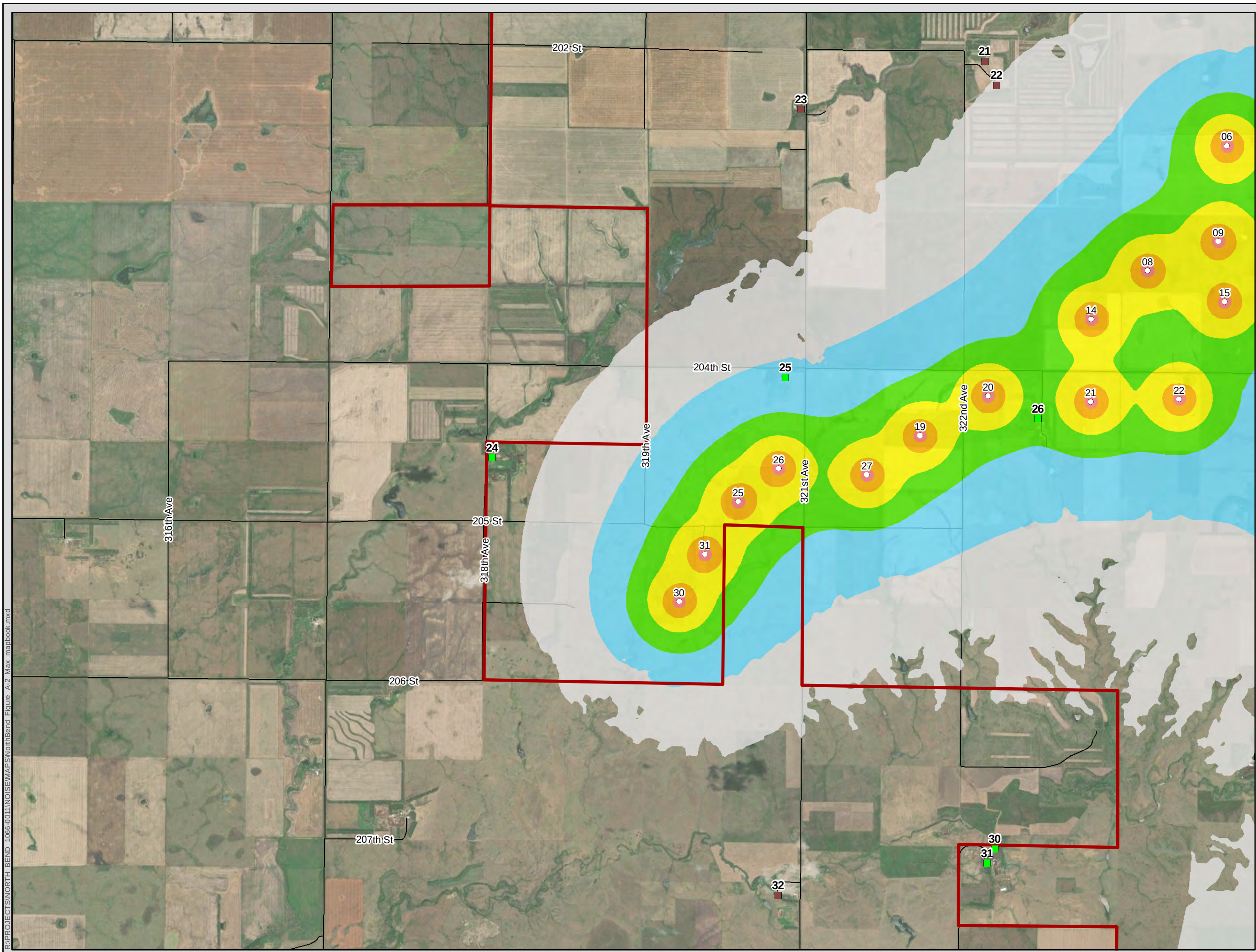
Figure A-2C Received Sound Levels - Maximum Wind Turbine Rotational Speed
