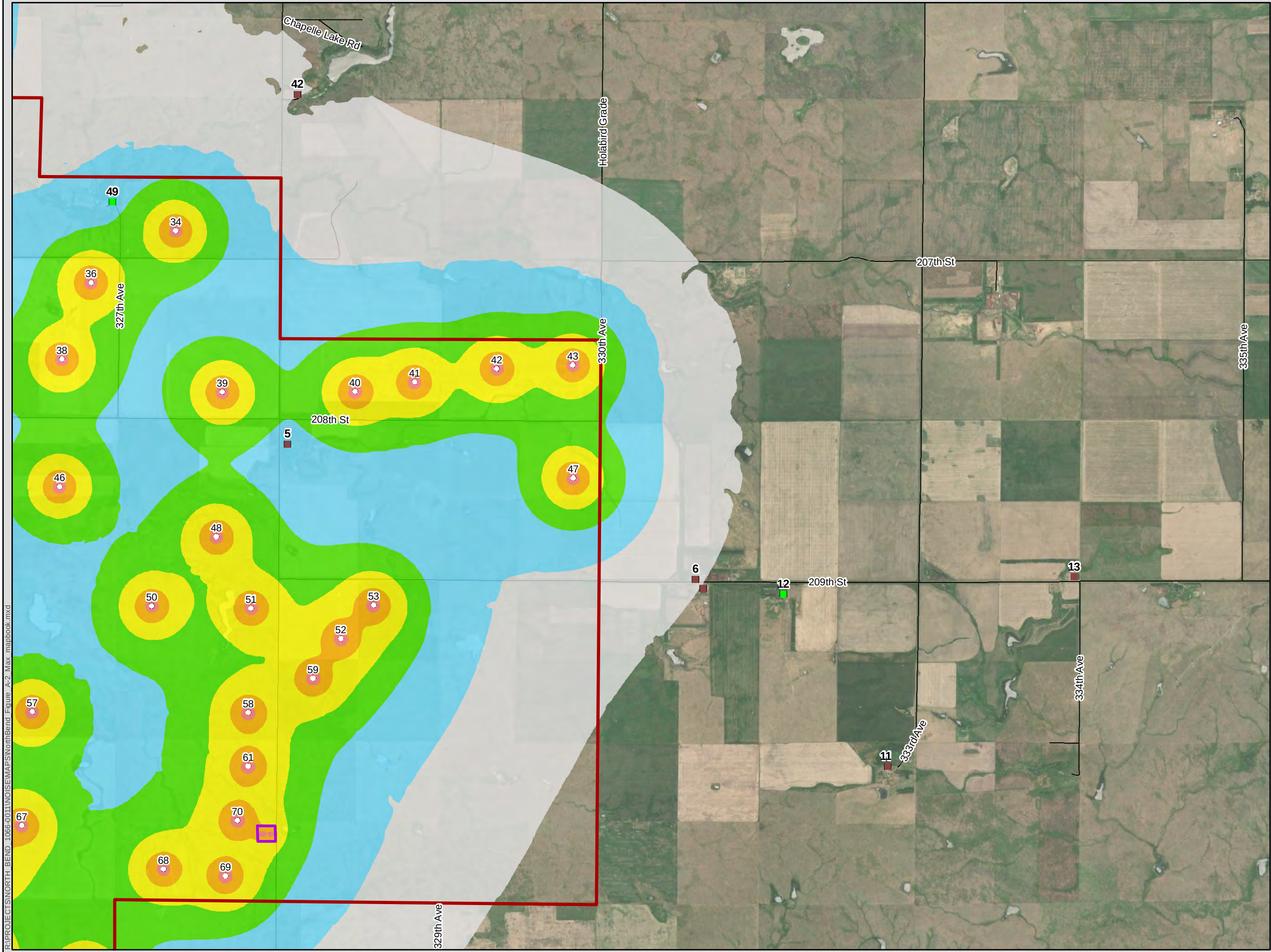
Figure A-2F Received Sound Levels - Maximum Wind Turbine Rotational Speed
