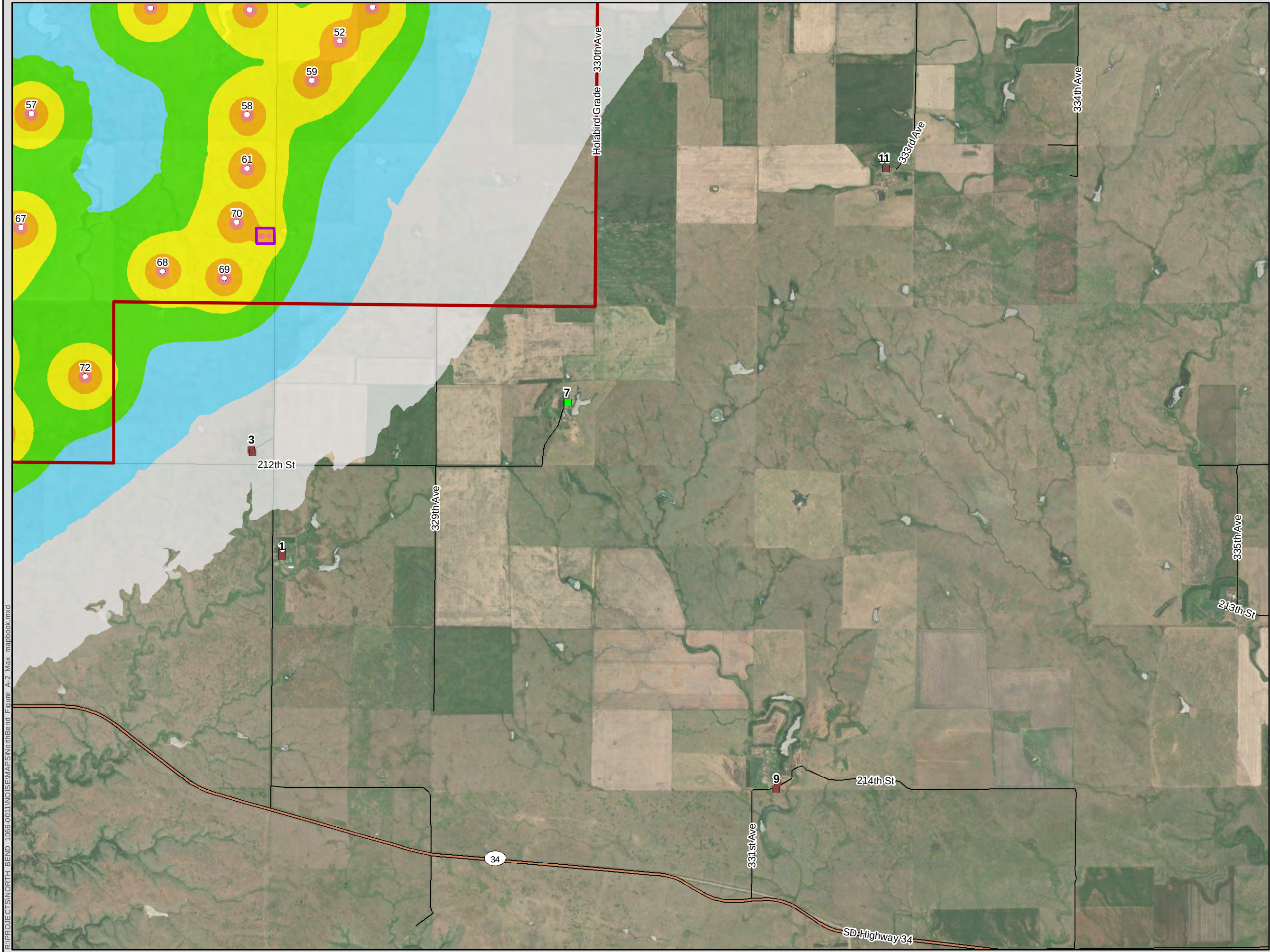
Figure A-2H Received Sound Levels - Maximum Wind Turbine Rotational Speed
