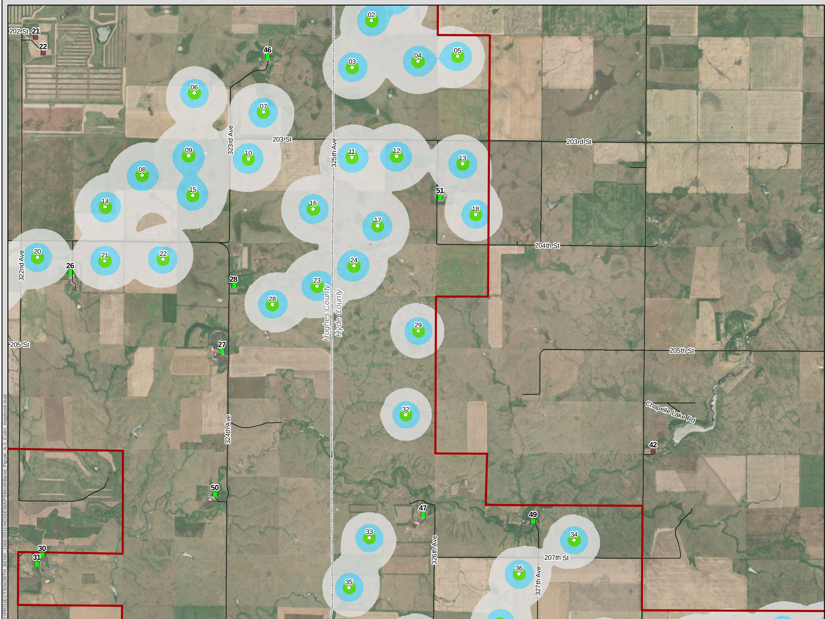
Figure A-1D Received Sound Levels - Cut-in Wind Turbine Rotational Speed
