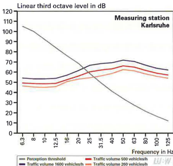
Figure 5.2-3: Third octave spectra, measuring station Karlsruhe
