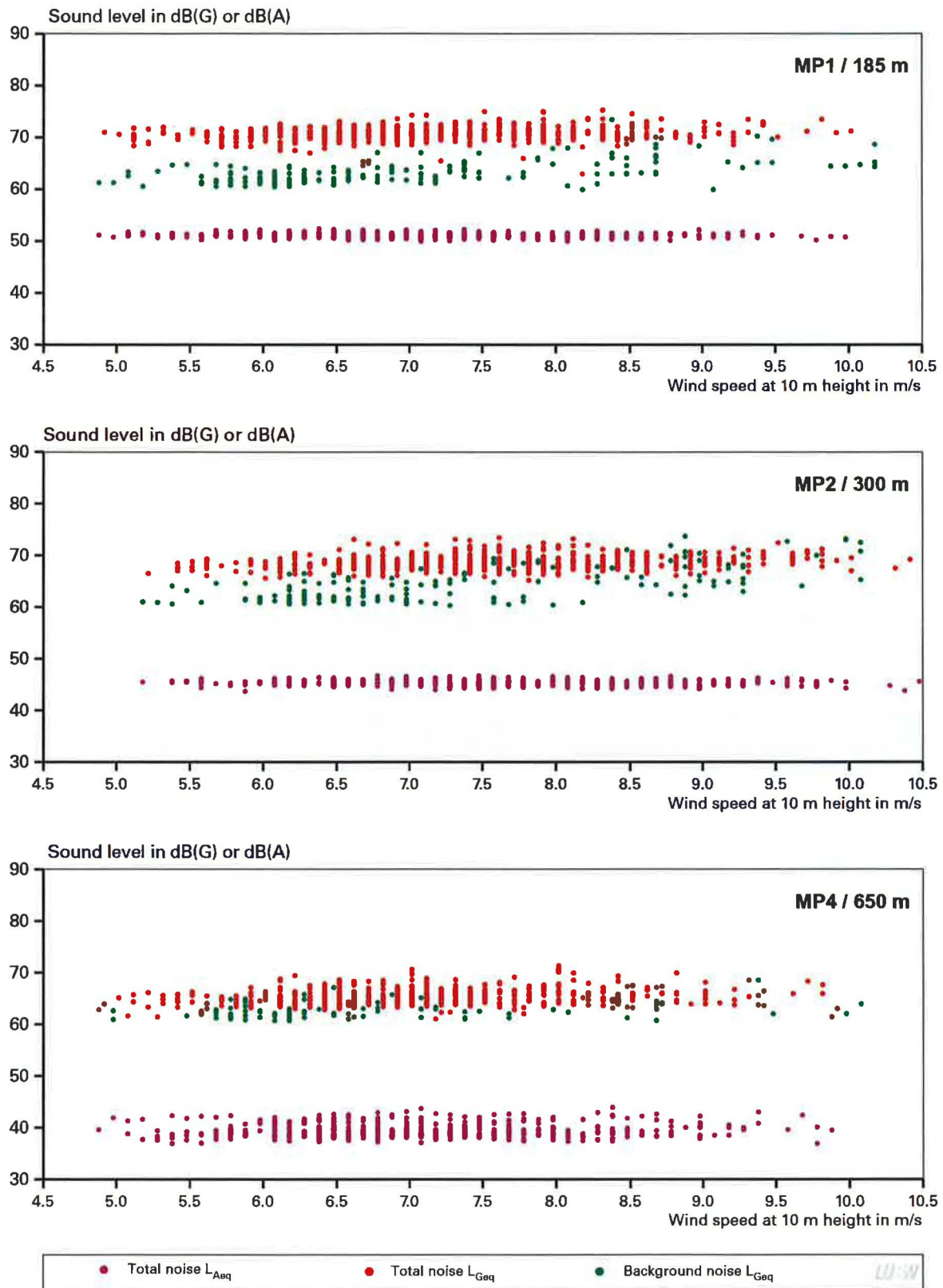
Figure 4.6-8: Audible sound level (A level) and infrasound level (G level) depending on the wind speed for the wind turbine WT 5. The G levels when the turbine is switched on (red dots) and when the turbine is switched off (green dots) are shown, as are the A levels with the turbine switched on (violet dots).
