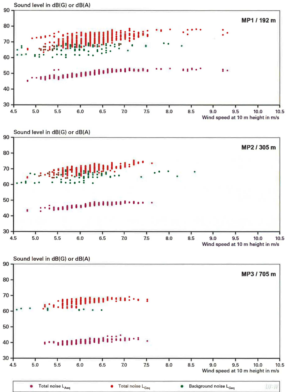
Figure 4.7-6: Audible sound level (A level) and infrasound level (G level) depending on the wind speed for the wind turbine WT 6. The G levels when the turbine is switched on (red dots) and when the turbine is switched off (green dots) are shown, as are the A levels with the turbine switched on (violet dots).
