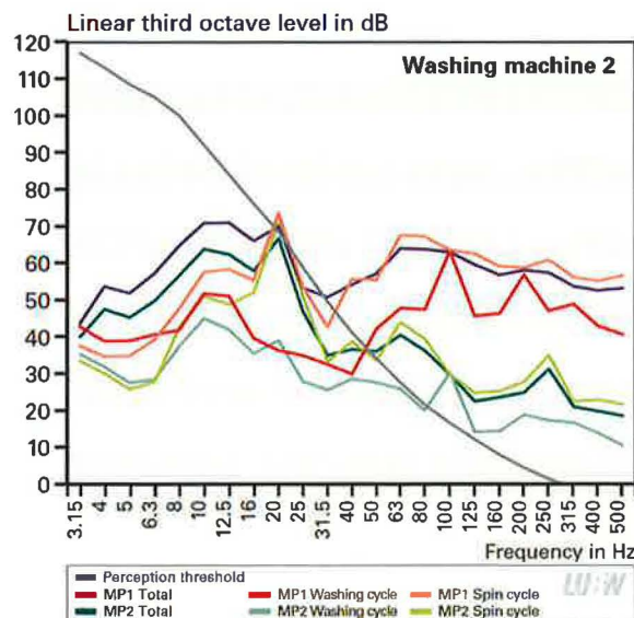
Figure 7.1-2: Third octave noise level of washing machine 2 at measurement points MP1 and MP2 for different operating states, with perception threshold according to Table A3-1 for comparison. "Total": Average level over the entire wash cycle.
