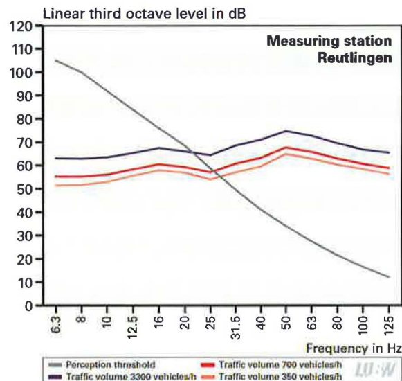
Figure 5.2-4: Third octave spectra, measuring station Reutlingen
