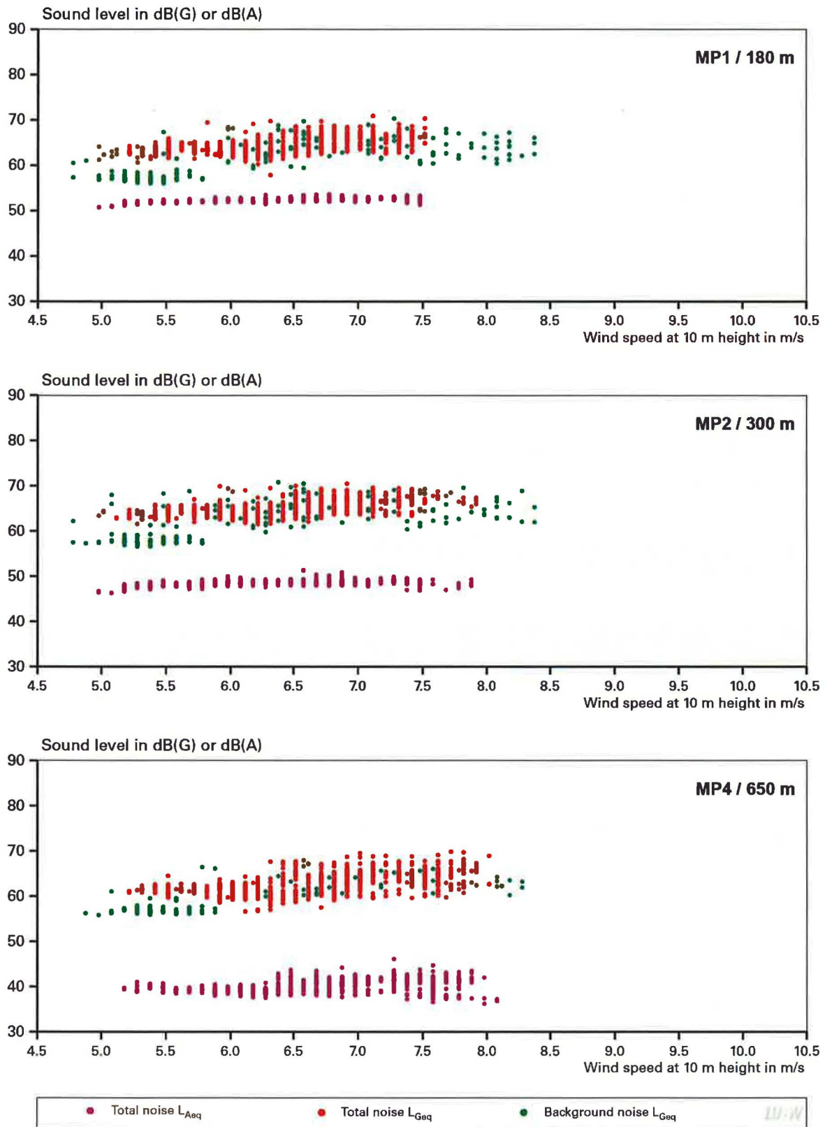
Figure 4.5-12: Audible sound level (A level) and infrasound level (G level) depending on the wind speed for the wind turbine WT 4. The G levels when the turbine is switched on (red dots) and when the turbine is switched off (green dots) are shown, as are the A levels with the turbine switched on (violet dots).
