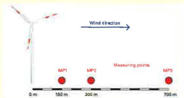
Exemplary measuring arrangement (not to scale)
