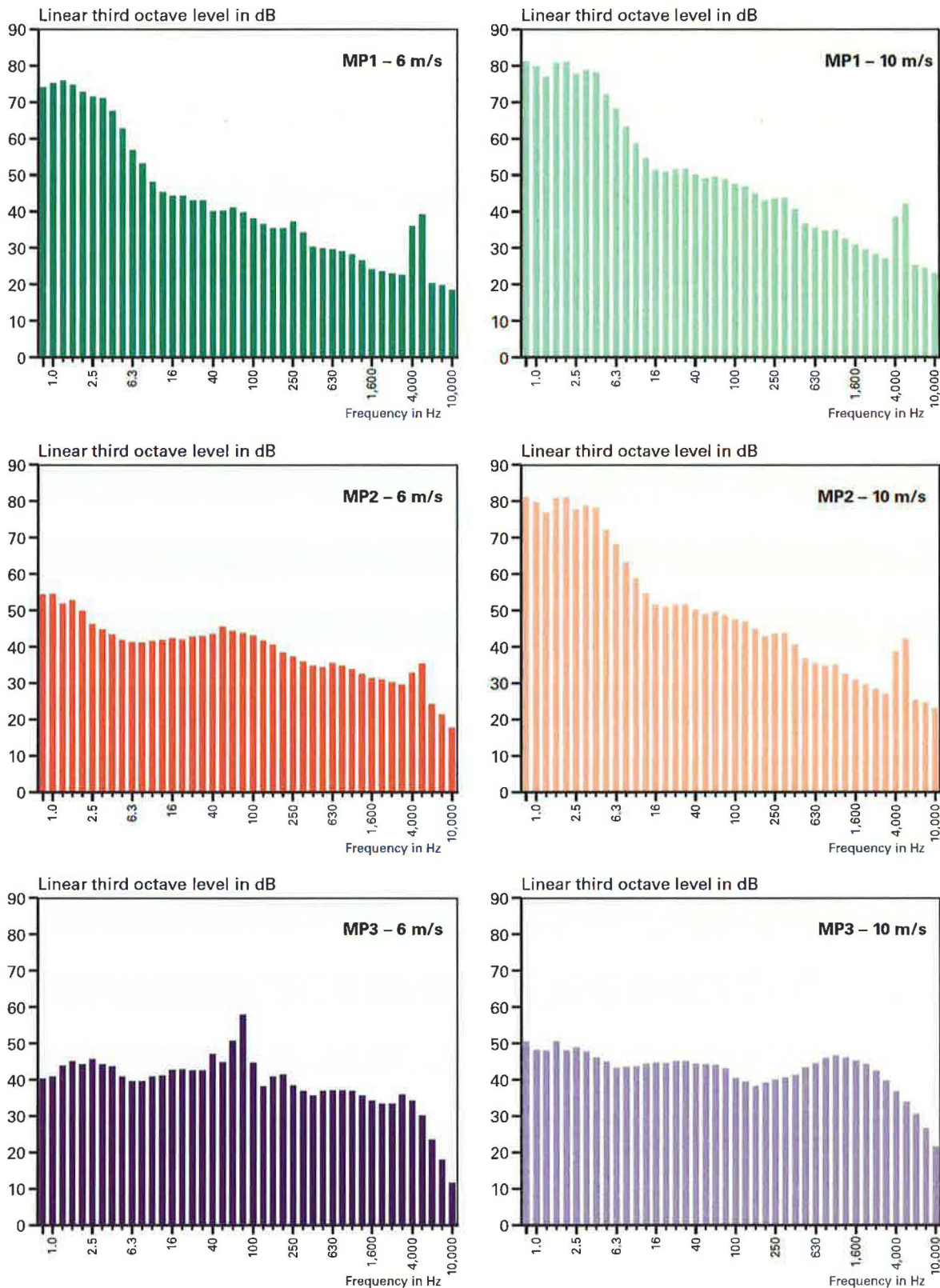
Figure 8.1-5: Third octave spectra of the background noise at the measurement point MP1 (open field), MP2 (edge of forest), and MP3 (forest). Left column: Wind speed 6 m/s; right column: Wind speed 10 m/s. The wind measurement was always carried out at the measurement point MP1 (open field).
