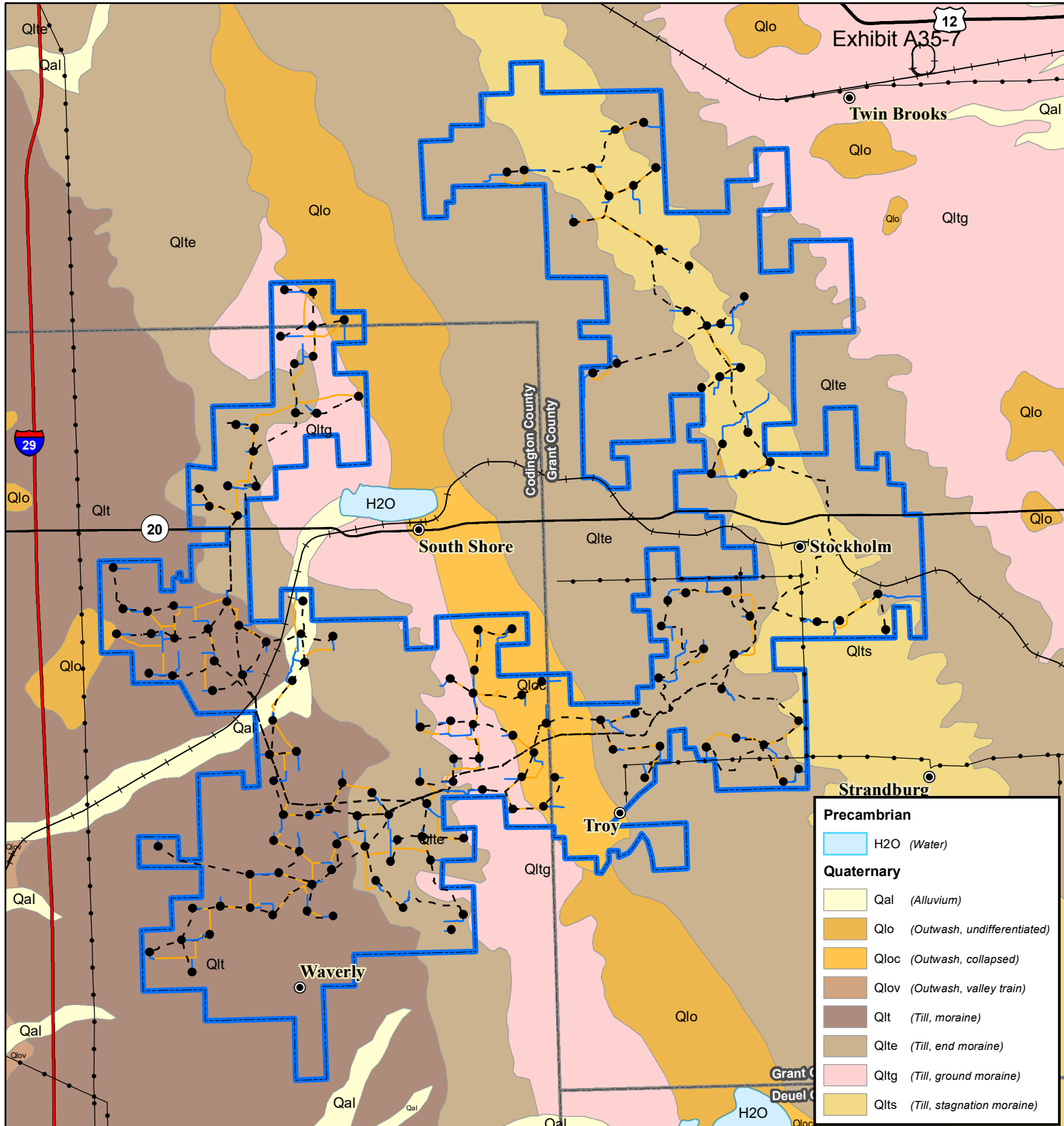
Figure 9a. Surficial Geology Crowned Ridge Wind Farm ● City ● Turbine — Access Road - - - Collector Line — Crane Path ●— Electrical Line —+— Railroad — Interstate Highway — U.S. Highway — State Highway ▭ Project Boundary ▭ County Boundary
