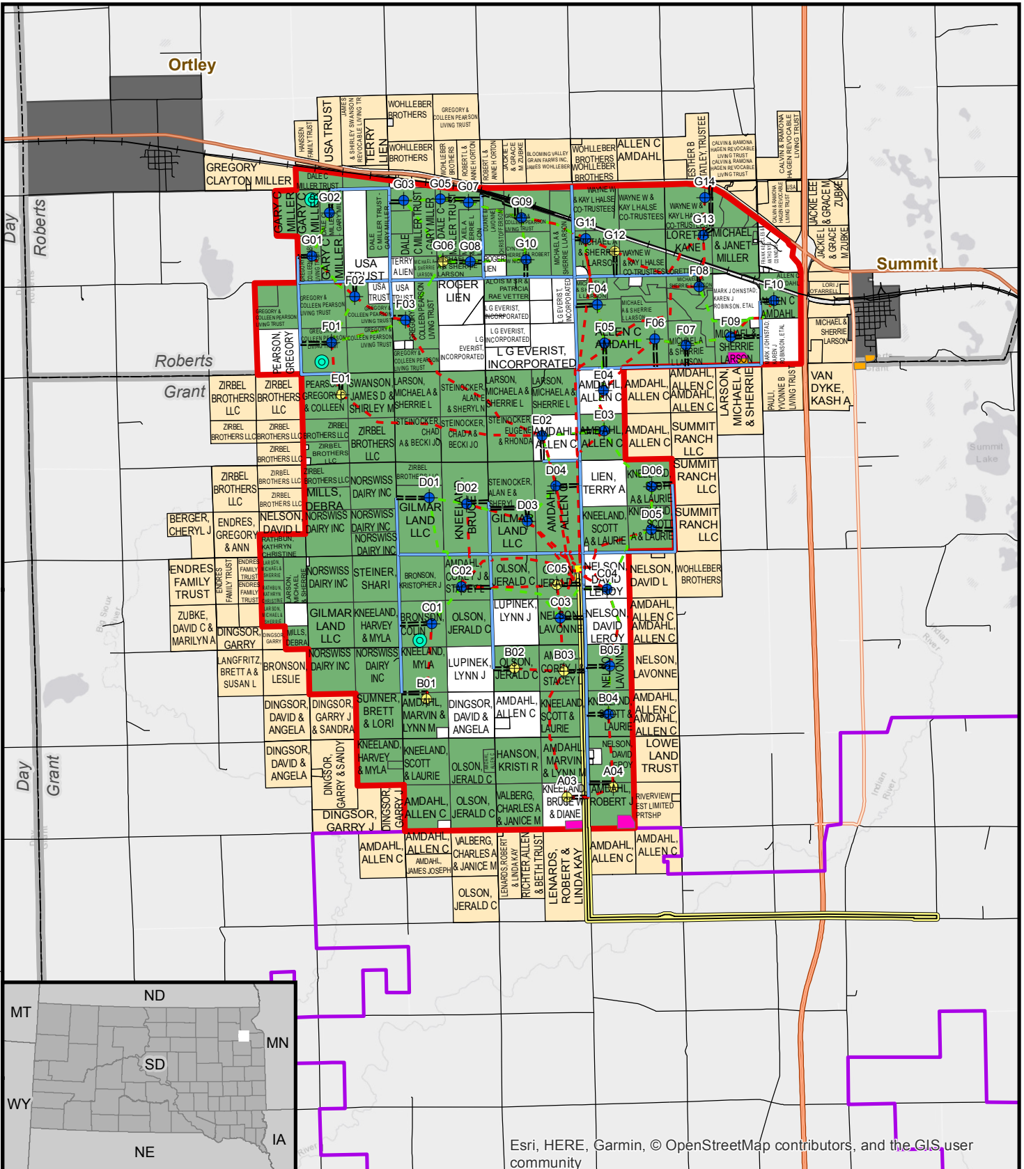
FIGURE 2: PROJECT LAYOUT DAKOTA RANGE III WIND ENERGY FACILITY & TRANSMISSION LINE SDPUC APPLICATION
