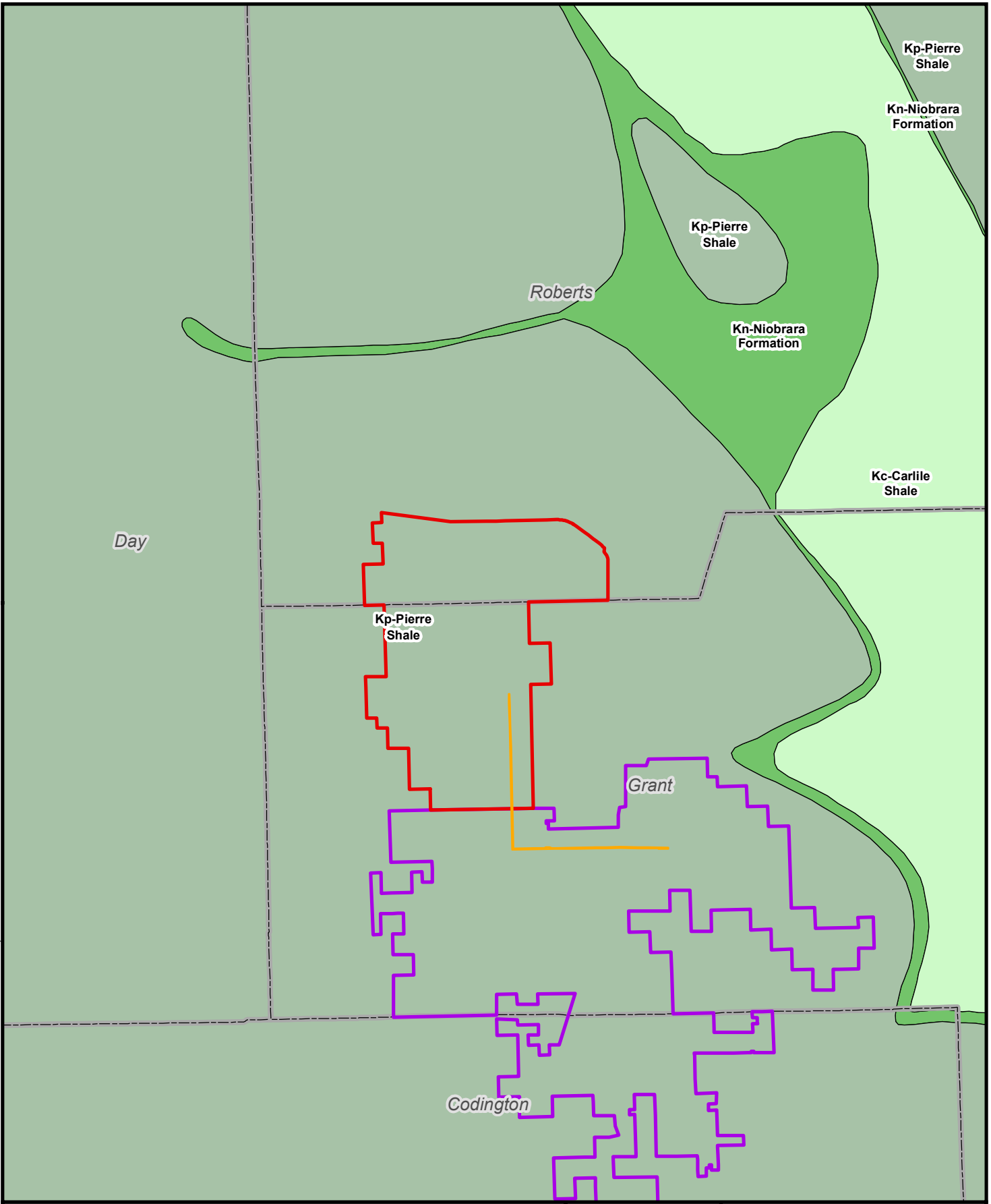
FIGURE 10: BEDROCK GEOLOGY DAKOTA RANGE III WIND ENERGY FACILITY & TRANSMISSION LINE SDPUC APPLICATION
