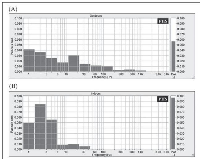
Figure 10. (A) Outdoor and (B) indoor sound pressure in Pascals
