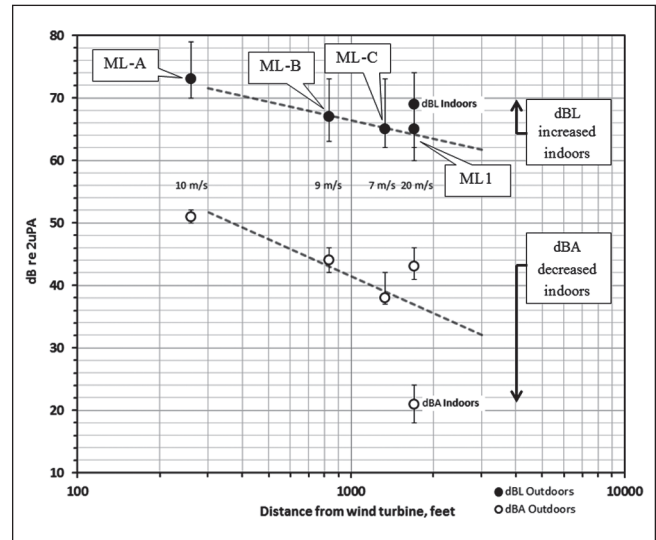
Figure 8. NOTUS root mean square (RMS) sound level versus distance
