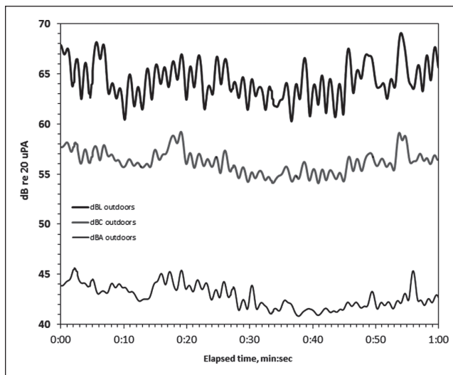
Figure 13. Outdoors sound levels: NOTUS "ON" (April 18, 2011)
