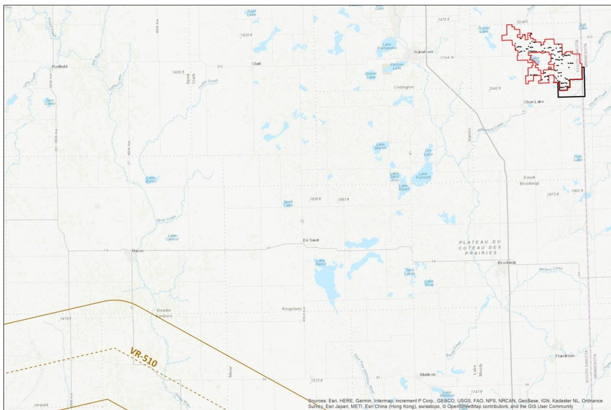
Figure 10: Military training routes in proximity to the Deuel Harvest wind project
