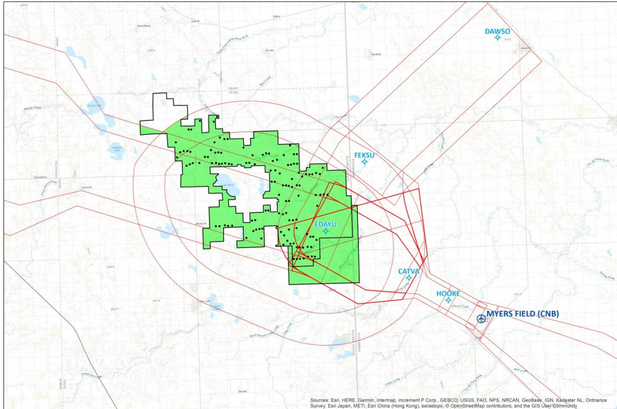
Figure 5: Myers Field Airport (CNB) RNAV (GPS) Approach to Runway 12
