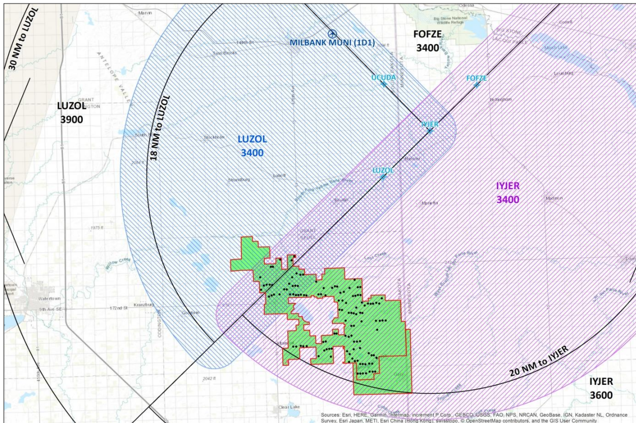
Figure 6: Milbank Municipal Airport (1D1) RNAV (GPS) Approach to Runway 31 TAA (black) with LUZOL 18NM (hatched blue) and IYJER 20NM (hatched purple) obstacle evaluation areas
