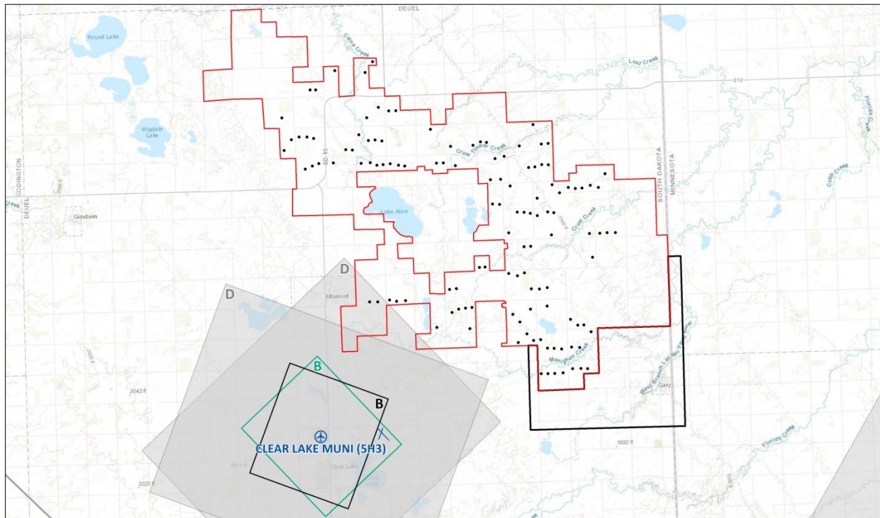
Figure 3: Clear Lake Municipal Airport (5H3) VFR traffic pattern airspace and the Deuel Harvest wind project
