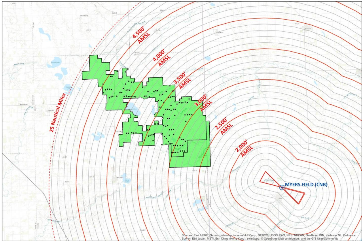
Figure 4: Myers Field (CNB) obstacle departure procedure assessment
