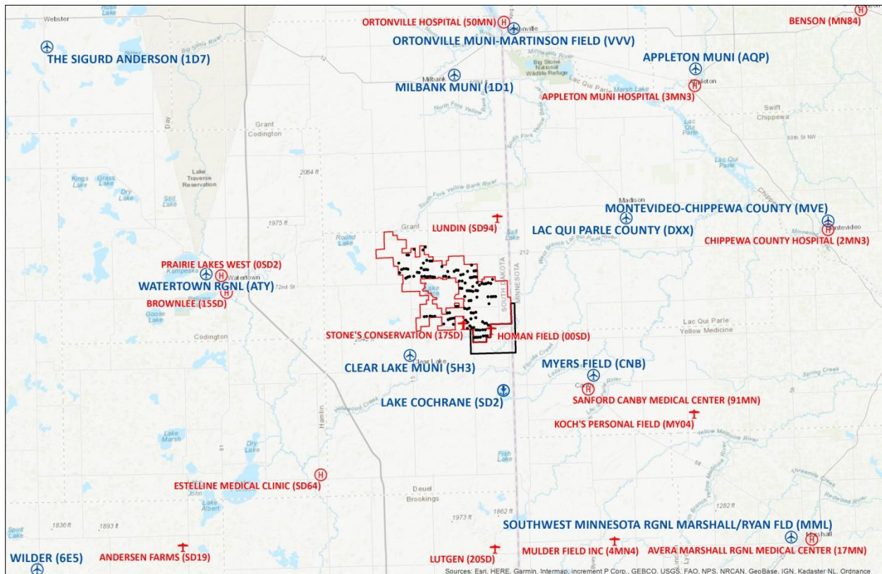
Figure 1: Public-use (blue) and private-use (red) airports and heliports in proximity to the Deuel Harvest wind project
