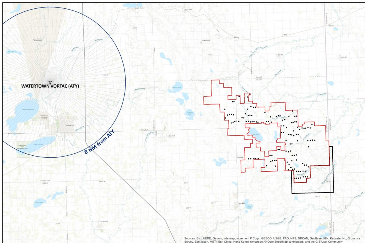
Figure 9: VOR protection areas in proximity to the Deuel Harvest wind project
