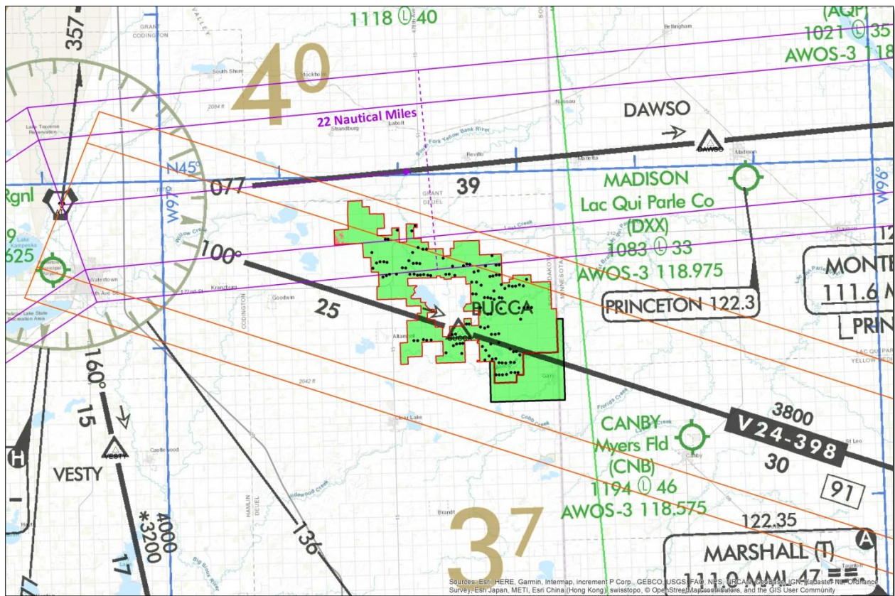
Figure 7: Low altitude enroute chart L-12 with V24-398 (orange) and V78 (purple) obstacle evaluation areas
