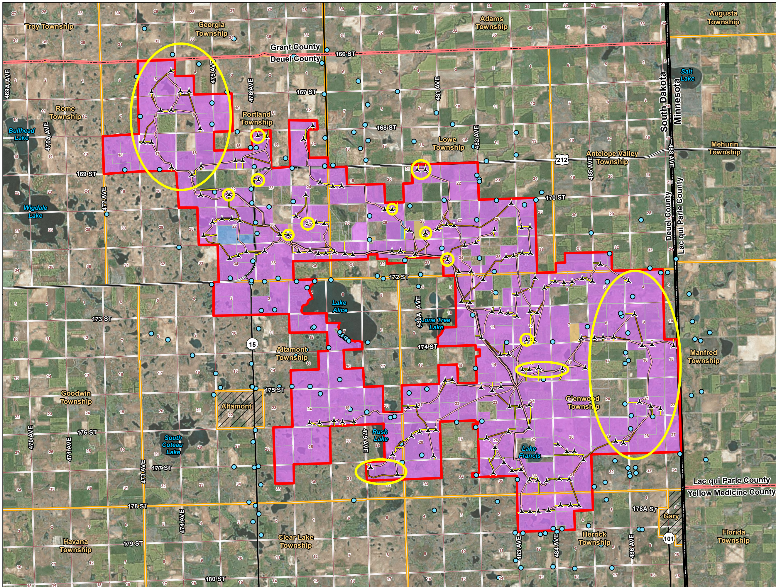
Figure 9 Changes to Proposed Turbine Locations from December 2017 Application for Consolidated Wind Energy System & Special Exception Permit Application Deuel Harvest North Wind Farm Deuel County, SD Invenergy For Permitting Review Purposes Only Date Created: 1/22/2017
