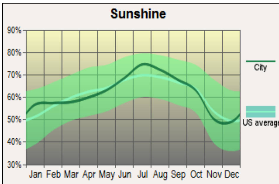
Figure 1: Monthly Sunshine Probability for Wagner, South Dakota
