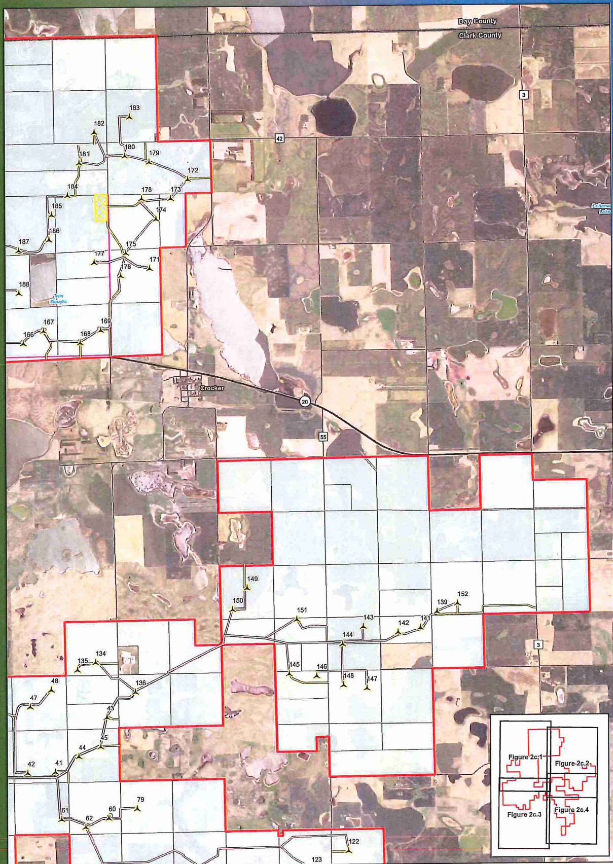
Figure 2c.2 Preliminary Project Layout Map Series GE 2.5-116
