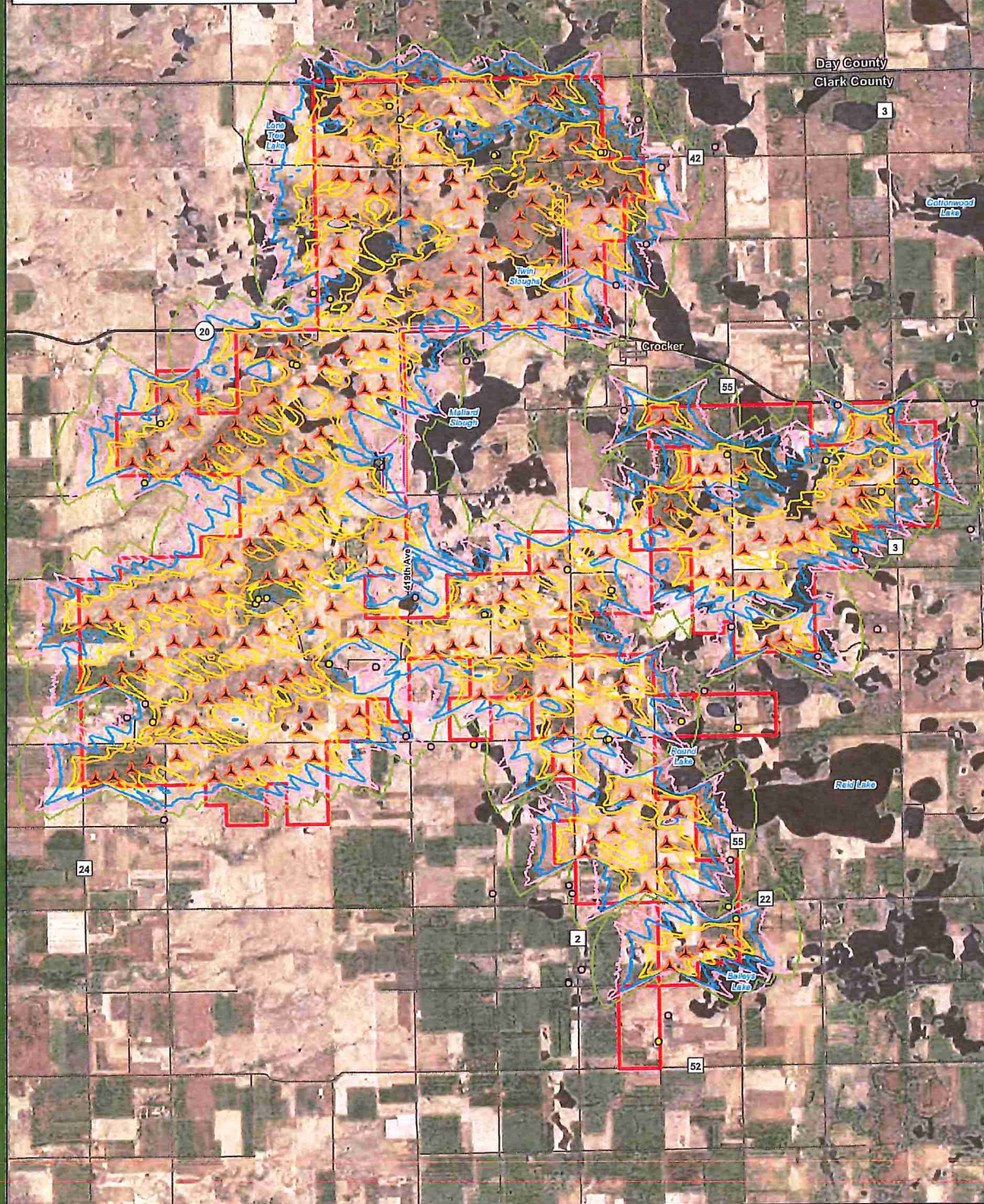
Figure 9d Shadow Flicker Vestas V110
