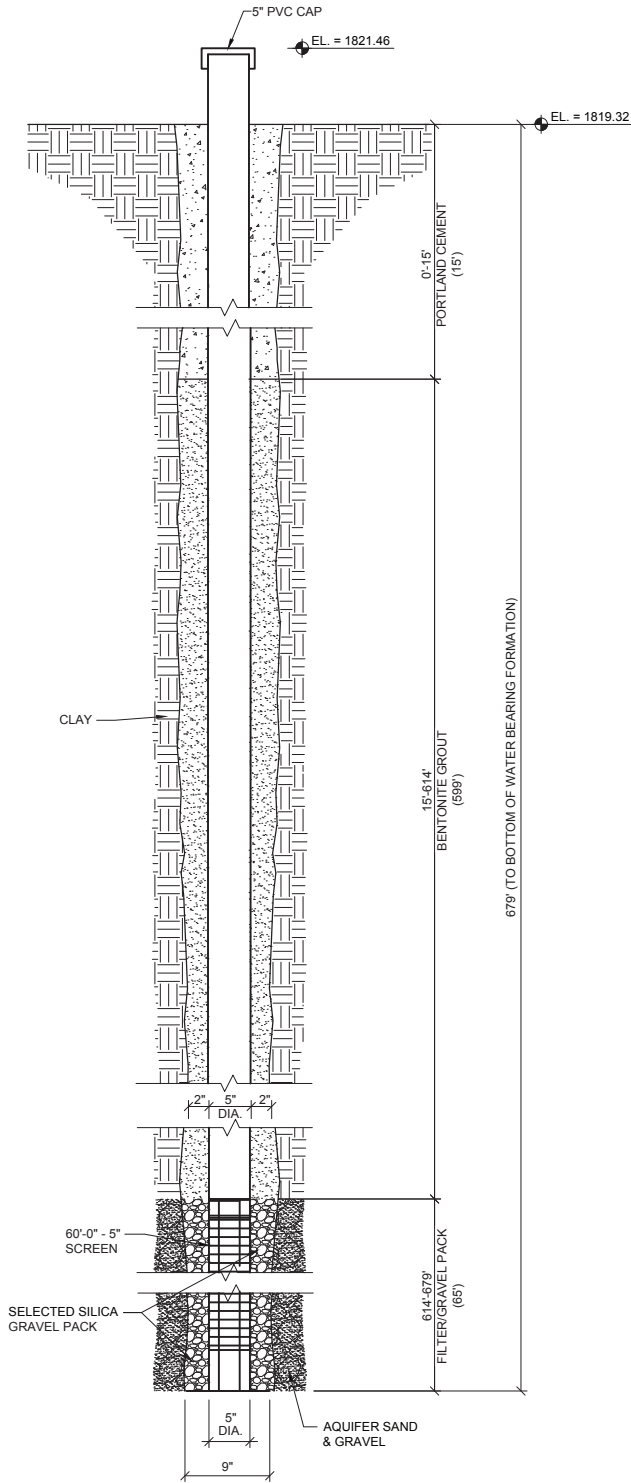
1 WELL SECTION 1 SCALE: NOT TO SCALE
