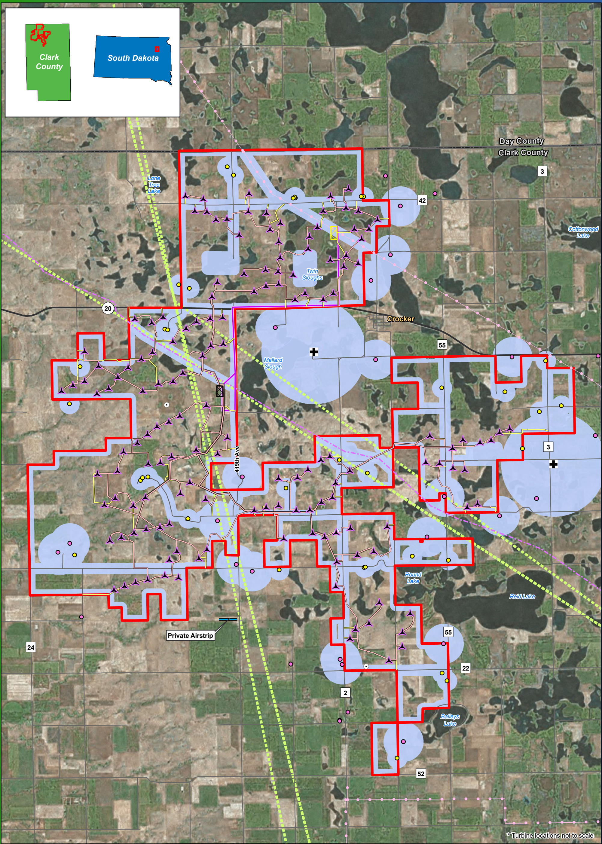
Figure 10a Project Layout and Constraints Gamesa G126
