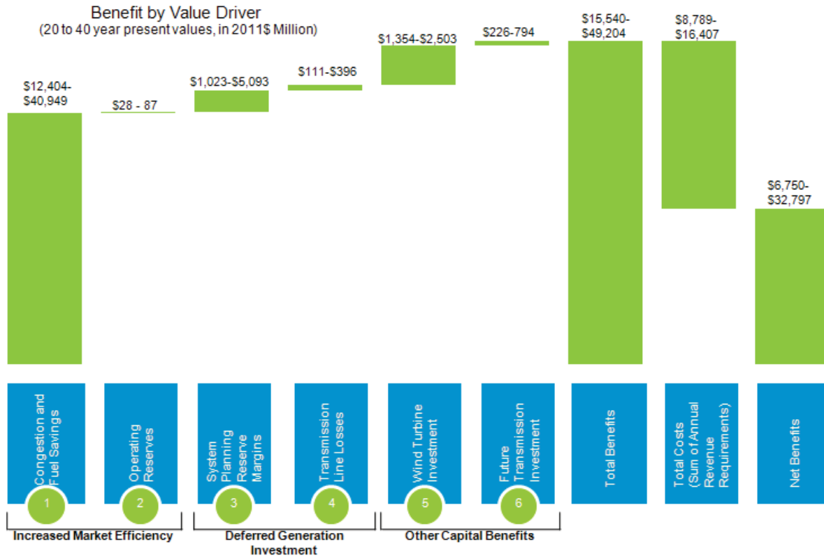
Figure 8.1: Recommended MVP portfolio economic benefits
