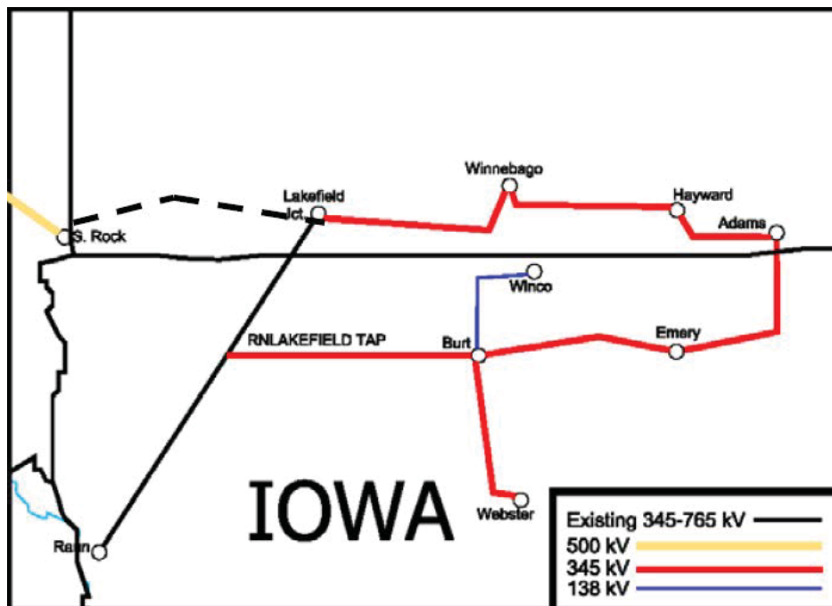
Figure 4.2: Iowa transmission identified in MTEP03
