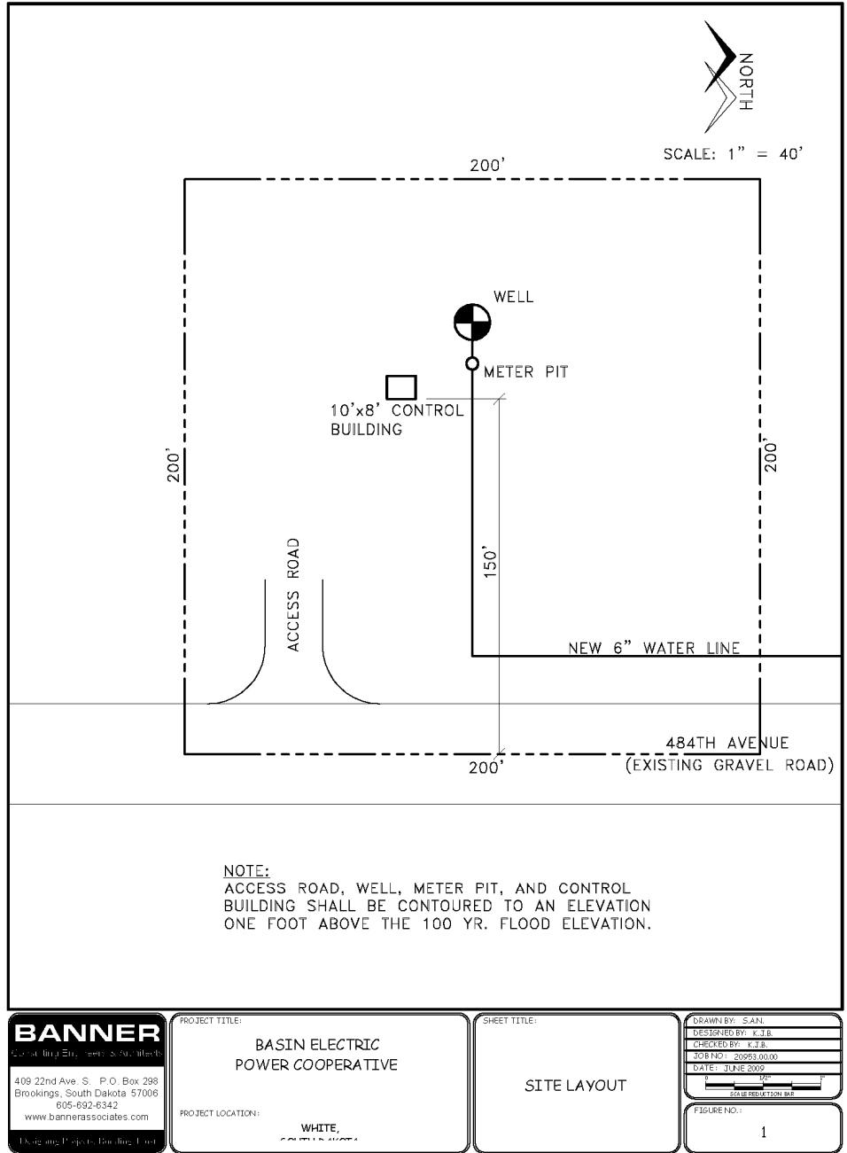
Exhibit 3.4-7: Typical Well Site Layout
