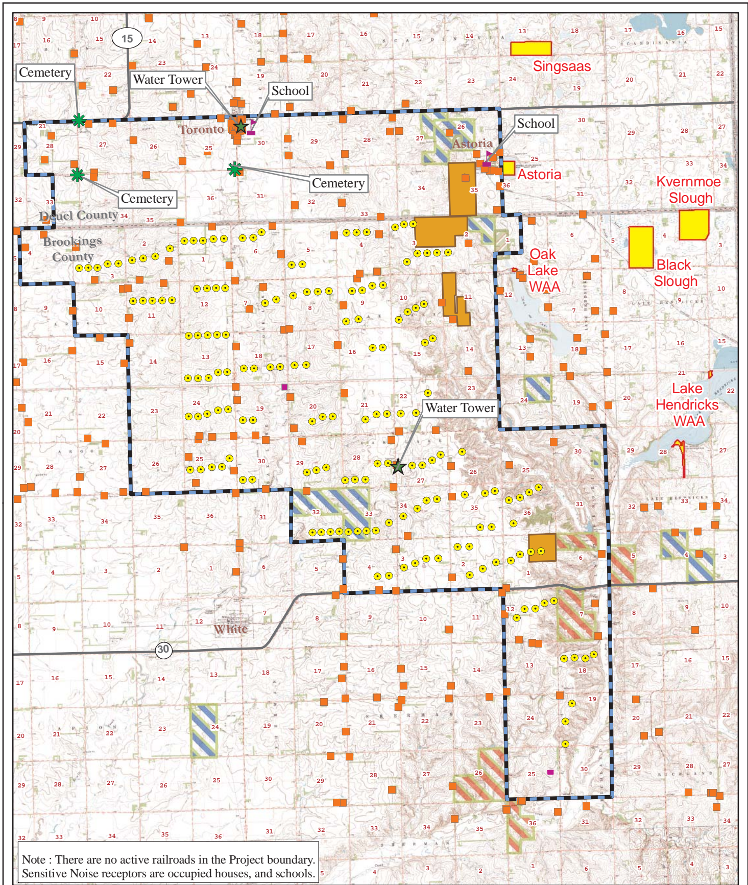
Figure 12a - Land Use & Public Lands, Wind Farm Facility Buffalo Ridge II Wind Farm Iberdrola Renewables Brookings and Deuel Counties, SD
