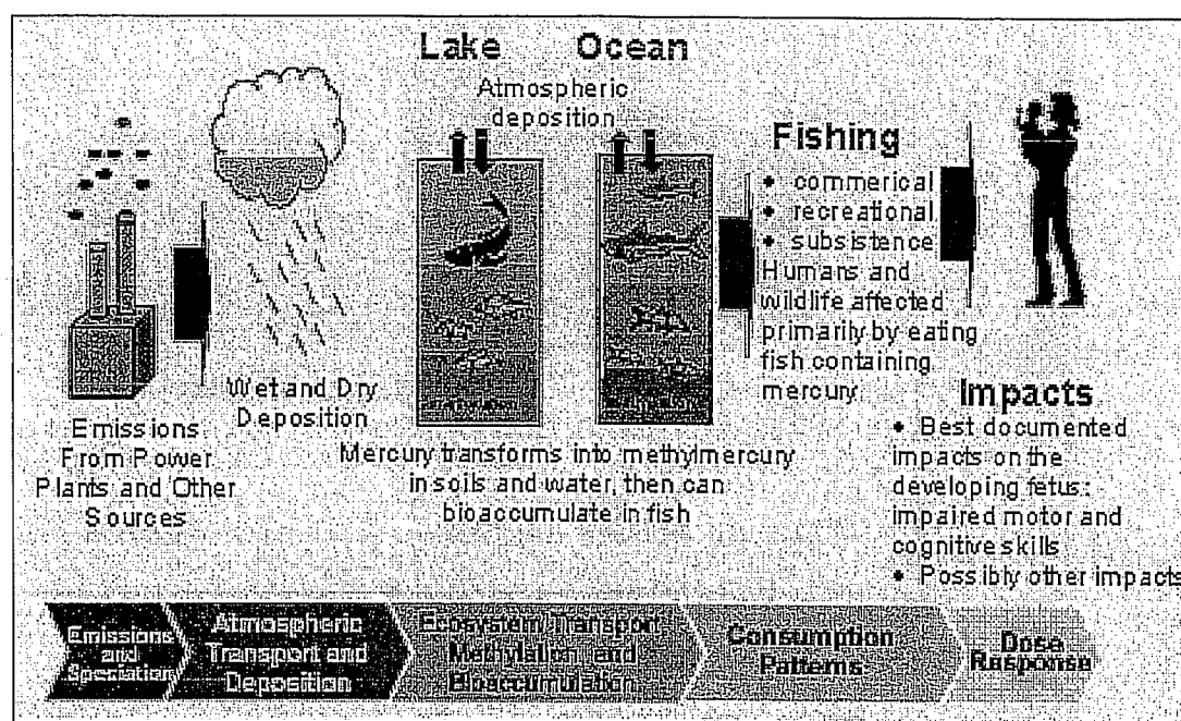
Figure 1-1: How Mercury Enters the Environment
