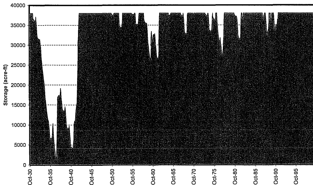
Figure 6: Water Storage Pond Storage Time Series: 38,000 Acre-Ft Pond with 12,000 Acre-Ft/Yr Consumption Rate
