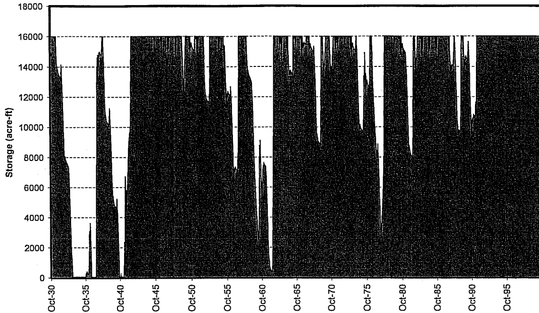
Figure 3: Water Storage Pond Storage Time Series: 16,000 Acre-Ft Pond with 12,000 Acre-Ft/Yr Consumption Rate
