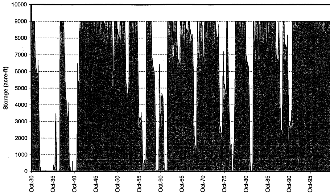
Figure 1: Water Storage Pond Storage Time Series: 9,000 Acre-Ft Pond with 12,000 Acre-Ft/Yr Consumption Rate
