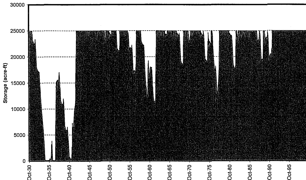
Figure 5: Water Storage Pond Storage Time Series: 25,000 Acre-Ft Pond with 12,000 Acre-Ft/Yr Consumption Rate
