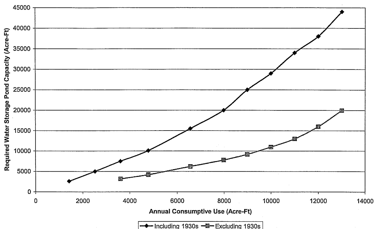
Figure 7: Required Water Storage Pond Capacity as a Function of Annual Consumptive Use
