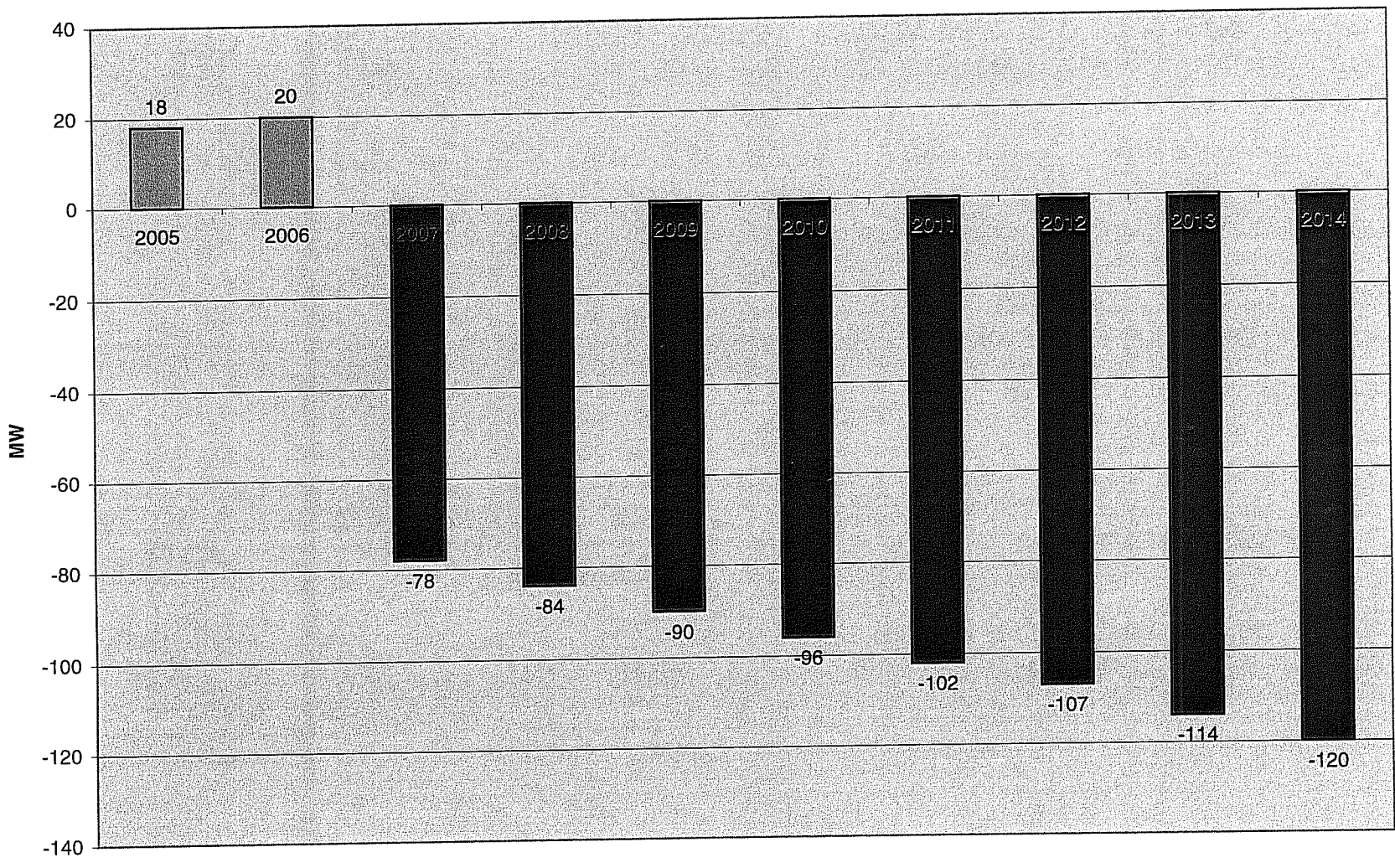
Exhibit 3-10 MDU SUMMER SURPLUS/DEFICIT FORECAST Big Stone II Project Big Stone II Co-owners
