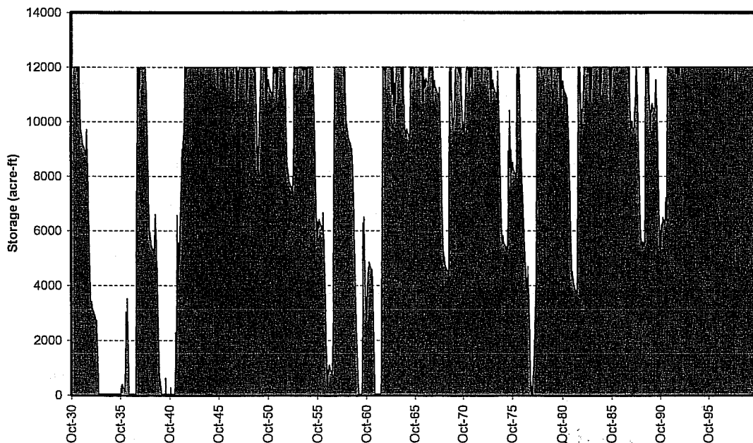
Figure 2: Water Storage Pond Storage Time Series: 12,000 Acre-Ft Pond with 12,000 Acre-Ft/Yr Consumption Rate
