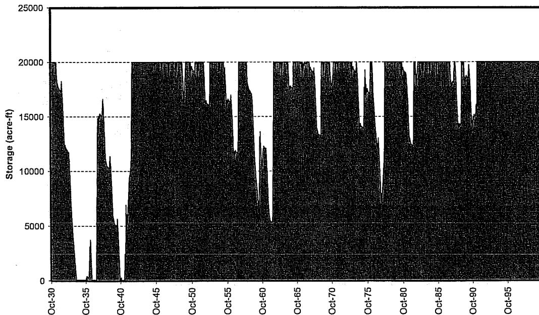
Figure 4: Water Storage Pond Storage Time Series: 20,000 Acre-Ft Pond with 12,000 Acre-Ft/Yr Consumption Rate
