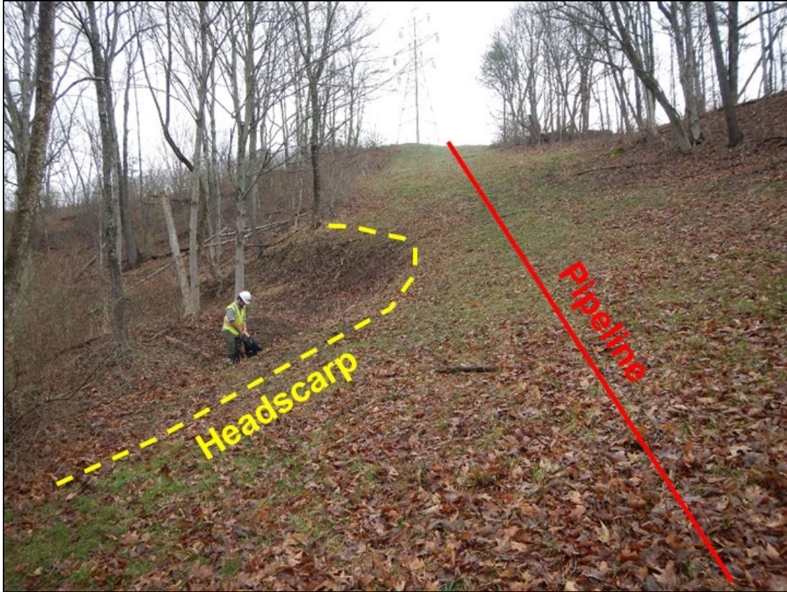
Figure 5-2. View showing a landslide headscarp (mapped during a Phase II) encroaching into the cleared ROW and approaching the pipeline centerline.
