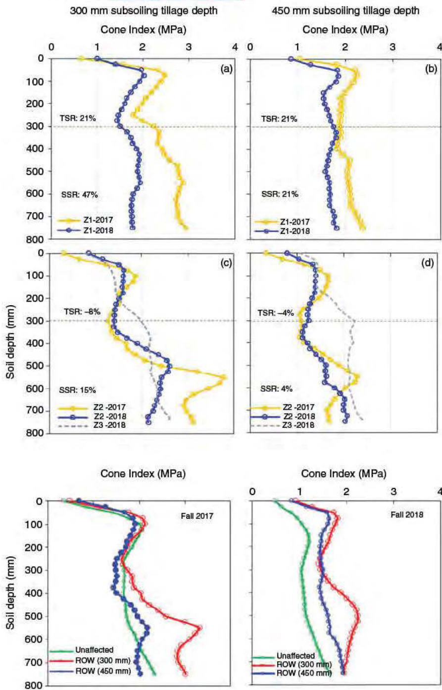
FIGURE 4 Soil cone penetration resistance profile for soils within trafficked ROW zones and unaffected zone from the fall 2017 and fall 2018 data. Within the ROW trafficked zones, subsoiling tillage treatments of 300 mm (a, c) and 450 mm (b, d) were applied. Dashed lines (at 300 mm) separate the top soil layers from the subsoil layers. TSR and SSR (%) represent soil strength improvement within the affected zones (i.e. Z1, Z2) comparing data from fall 2017 and fall 2018. In Z3, TSR and SSR were not calculated because data were not collected in fall 2017 [Colour figure can be viewed at wileyonlinelibrary.com ]
