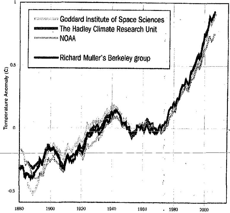
Temperature data obtained by three original sources contrasted with the data obtained by Richard Muller's Berkeley group
