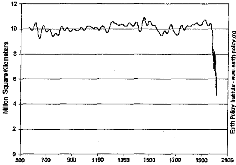
Late Summer Arctic Sea Ice Extent, 563-2012
