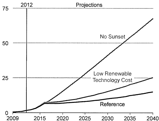
Figure MT-13. Residential distributed generation capacity in three cases, 2009-40 (gigawatts)
