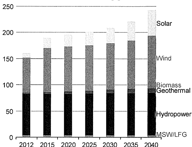
Figure MT-36. Renewable electricity generating capacity by energy source, including end-use capacity in the Reference case, 2012-40 (gigawatts)
