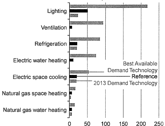
Figure MT-16. Efficiency gains for selected commercial equipment in three cases, 2040 (percent change from 2012 installed stock efficiency)
