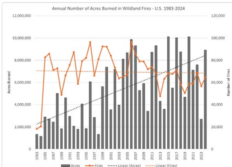
Figure 3: Increased size of wildfires and total acres burned, 1983-2024
