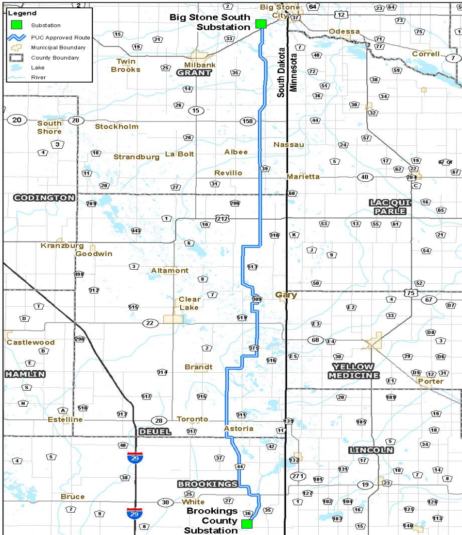
Figure 1: Proposed 345 kV line from Brookings to Big Stone South
