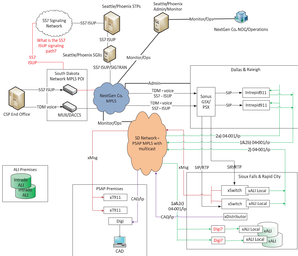
Figure 1 - South Dakota 911 Network
