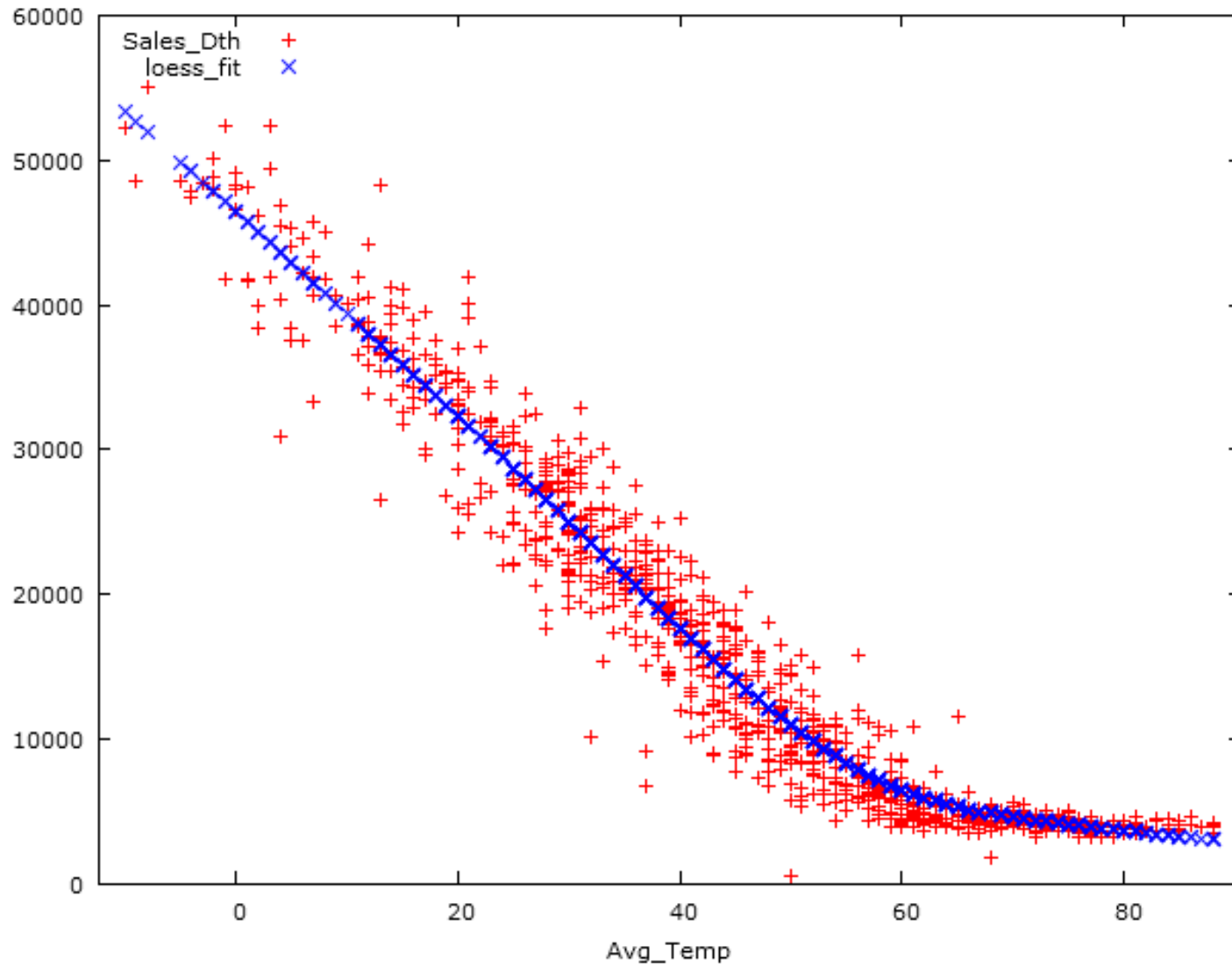
BLACK HILLS SYSTEM -- Average Temperature vs. Sales_Dth
