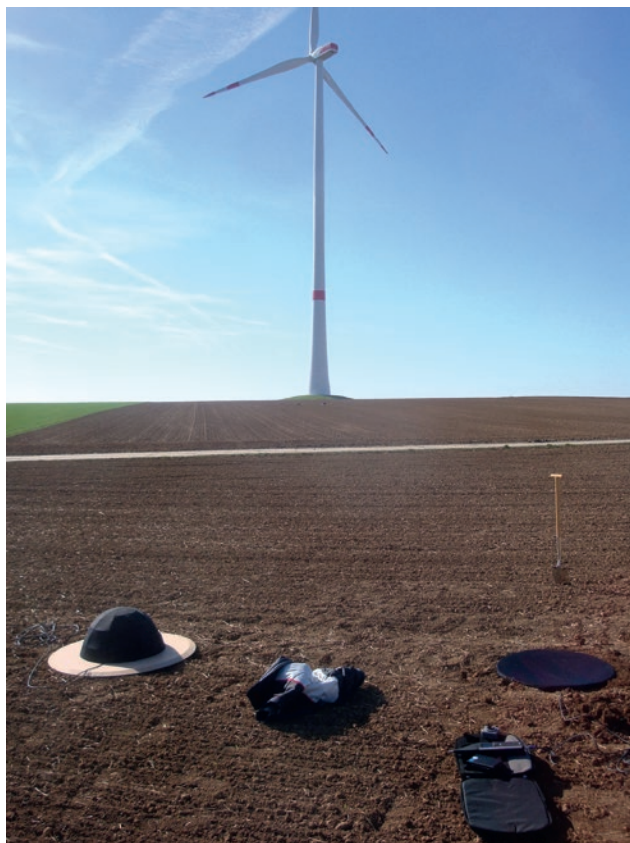
Figure 4.5-1 (right): Measurement points MP2 and MP3 at a distance of 300 m from the tower axis. Reverberant plate and double wind screen (left), spanned hole in the ground (right). Photo: Wölfel company
