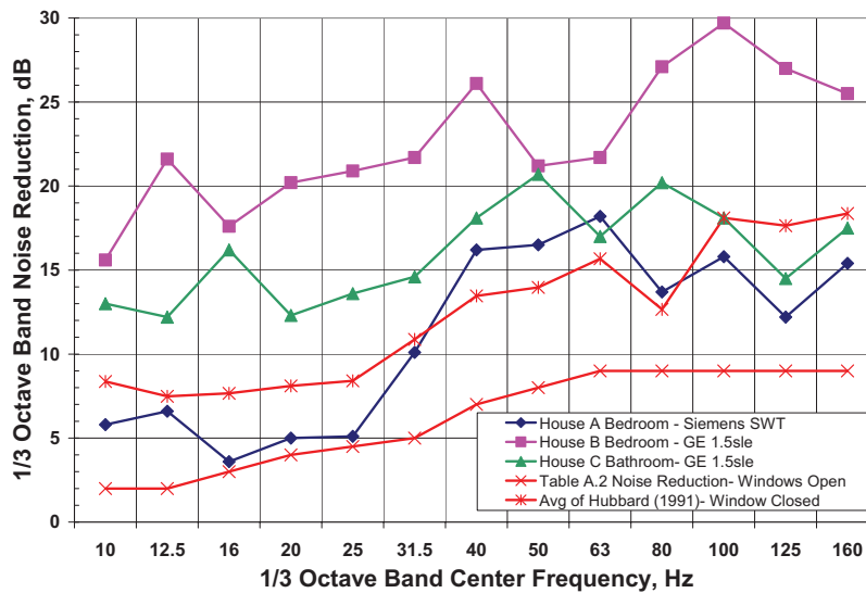
Fig. 19—One-third octave band interior noise reduction—Windows closed.
