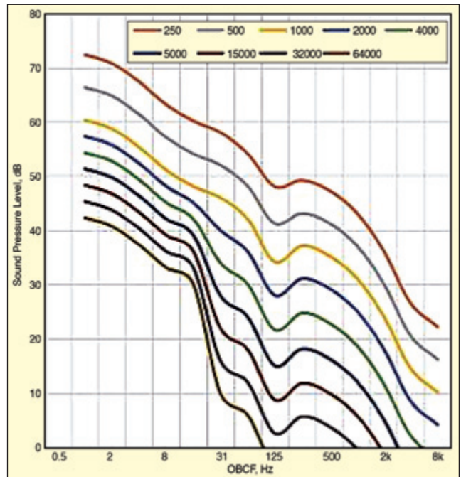
Figure 18. Calculated L_p spectra as function of distance.
