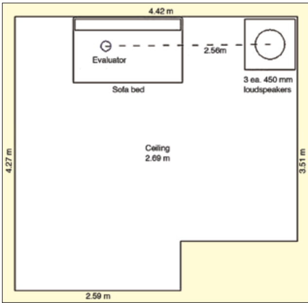
Figure 11. Layout of WTIS evaluation test room.
