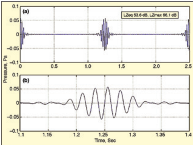
Figure 16. Wave-packet representation of third-spectrum lobe components.
