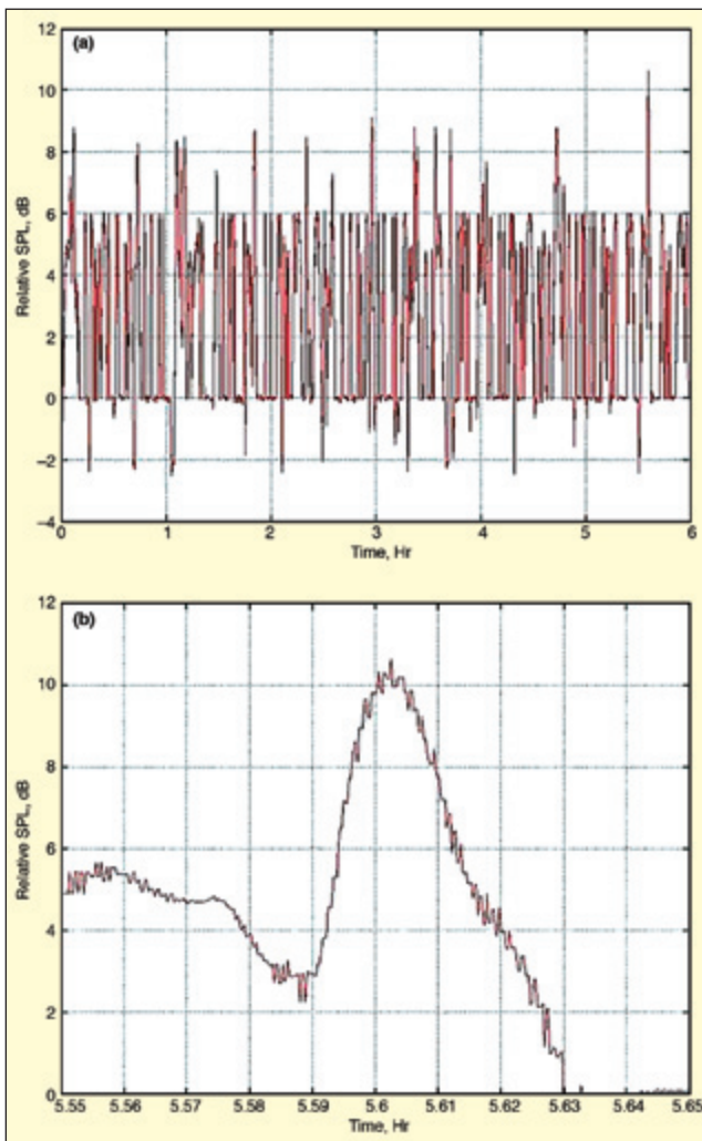
Figure 5. (a) Computed variations in SPL from a five-turbine array with unequal rotation rates relative to incoherent result; (b) expansion of largest peak.
