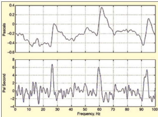
Figure 9. Shaft-order spectrum for wave shown in Figure 8.
