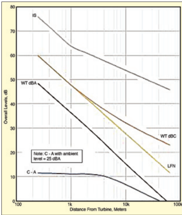
Figure 19. Overall levels as function of distance.
