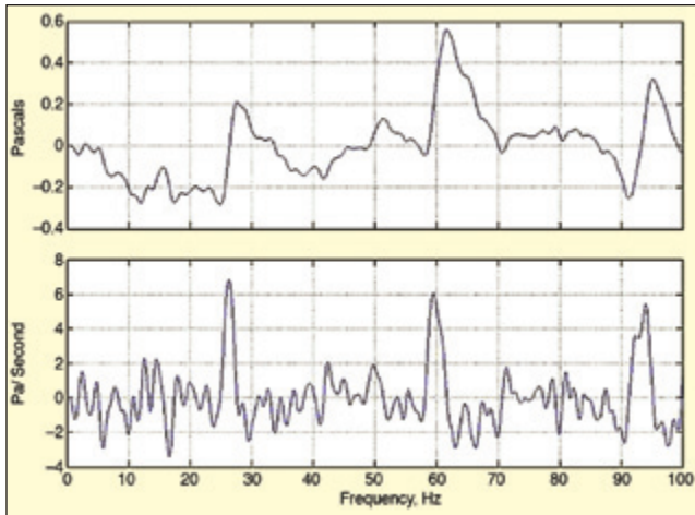
Figure 8. Example ensemble average waveform and time derivative with wind direction 60° re mic orientation.
