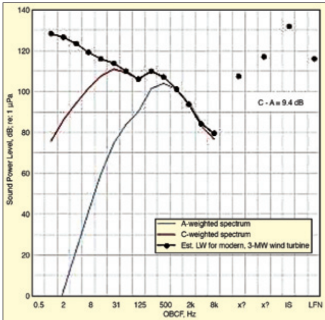
Figure 17. Typical spectrum from a large, modern, 3-MW wind turbine.
