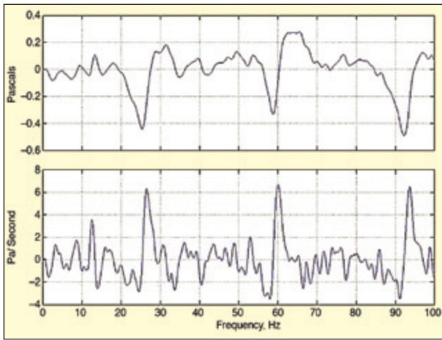
Figure 7. Example ensemble average waveform and time derivative with wind direction 140° re mic orientation.
