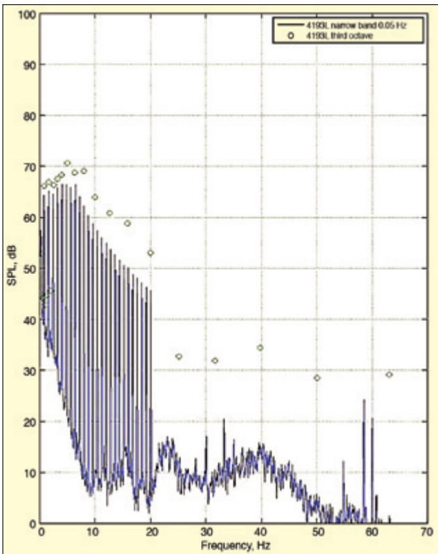
Figure 12. Generic WTIS spectrum used for initial evaluations.
