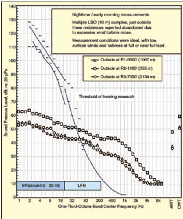
Figure 2. Typical wind turbine spectra and levels compared to threshold of hearing at low frequencies.
