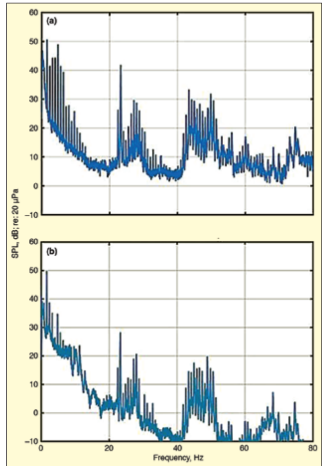
Figure 13. Outdoor (a) and indoor (b) spectra of WTN measured by Hansen.
