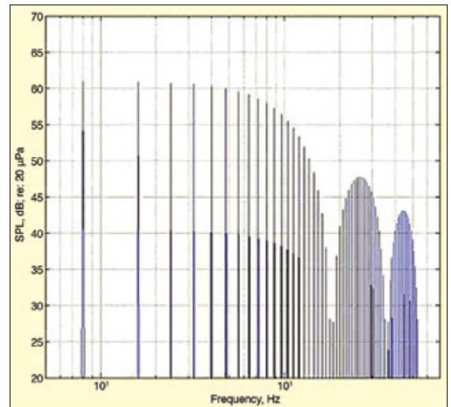
Figure 14. Spectrum of \sin(x)/x -weighted BPF harmonics.
