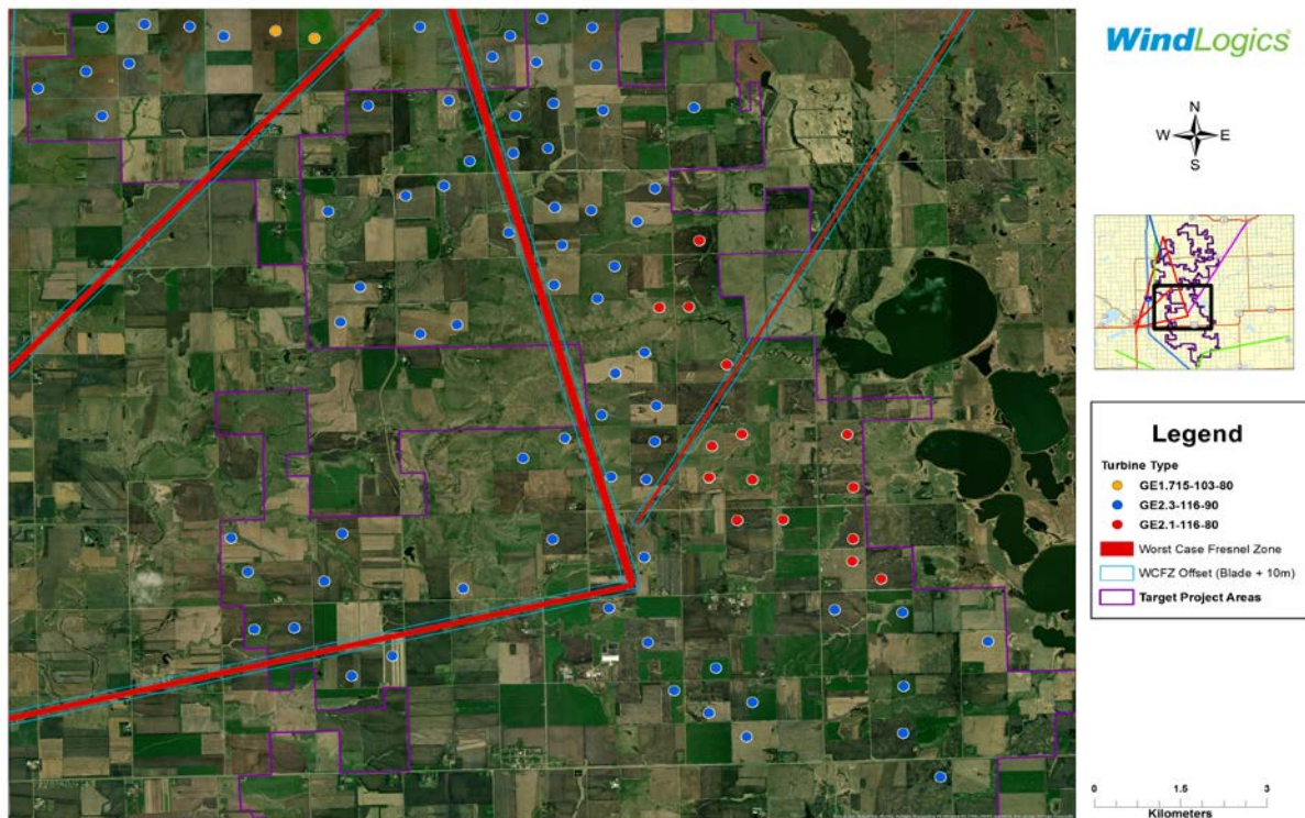
Figure 5: Crowned Ridge Wind Fresnel Zone Central
