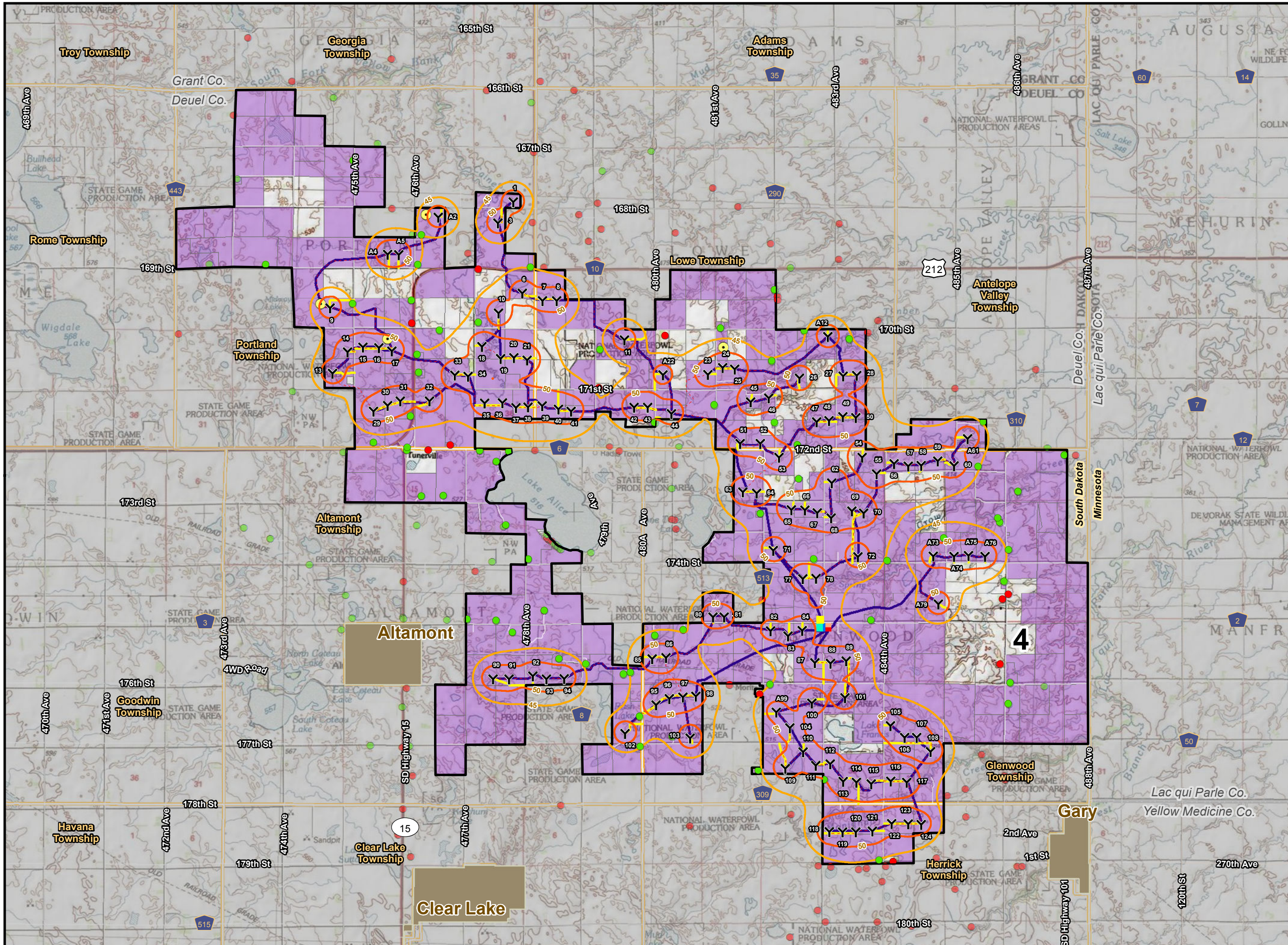
Figure D-2 Pre-Construction Wind Turbine Noise Analysis - Contour Map Deuel Harvest North Wind Farm Deuel Harvest Wind Energy LLC Deuel County, South Dakota
