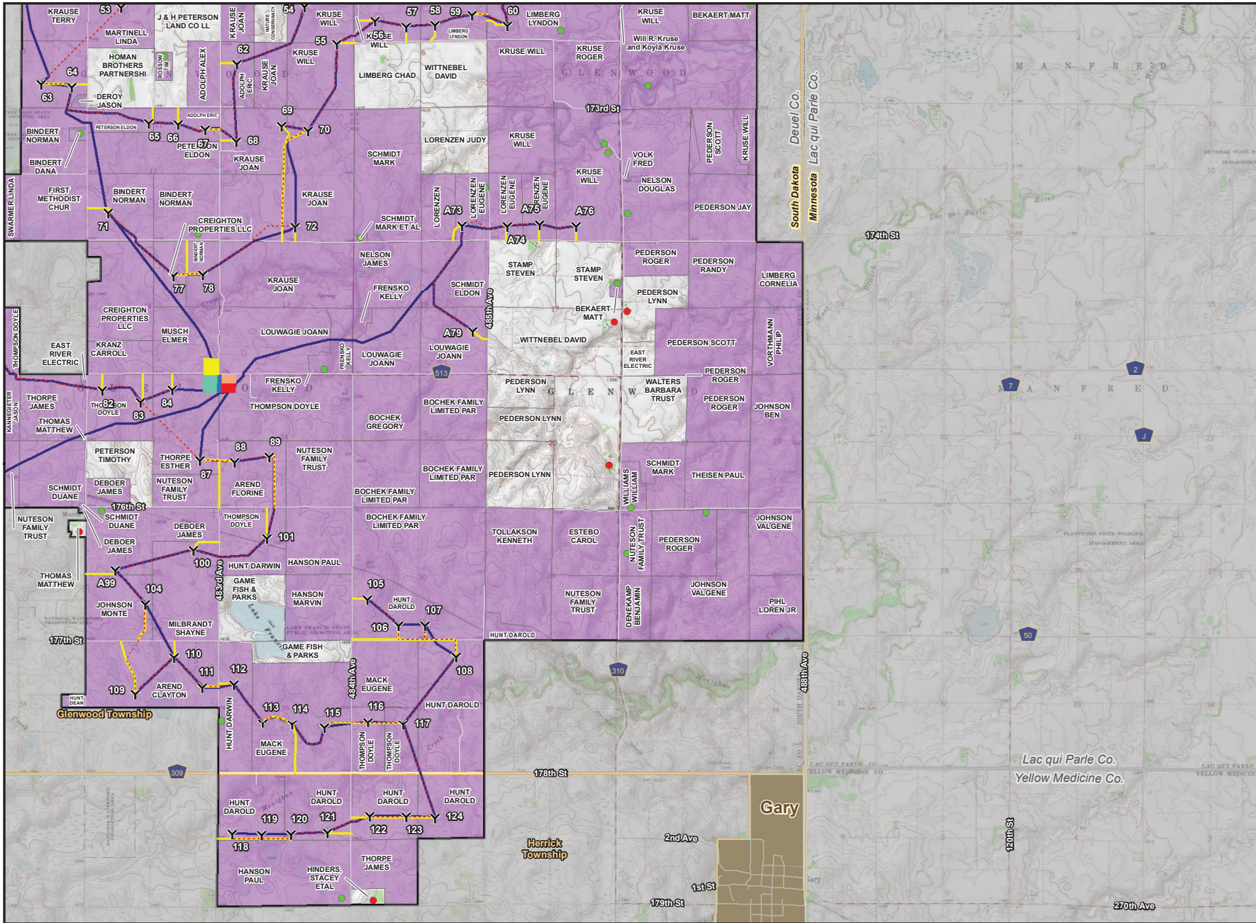
Figure A-4 Project Layout Deuel Harvest North Wind Farm Deuel Harvest Wind Energy LLC Deuel County, South Dakota Page 4 of 4
