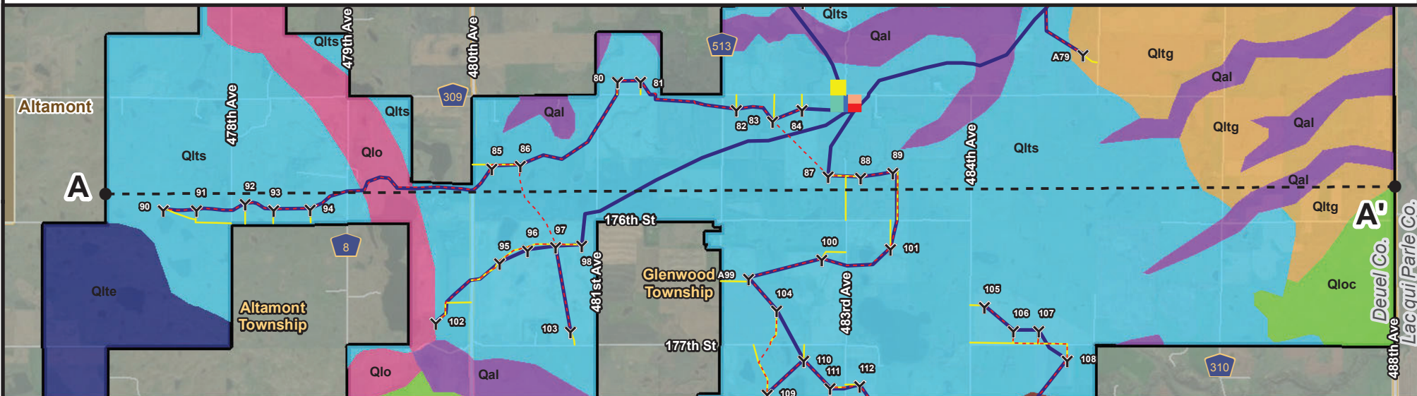
Figure A-10 Surficial Geology Cross Section A-A' Deuel Harvest North Wind Farm Deuel Harvest Wind Energy LLC Deuel County, South Dakota
