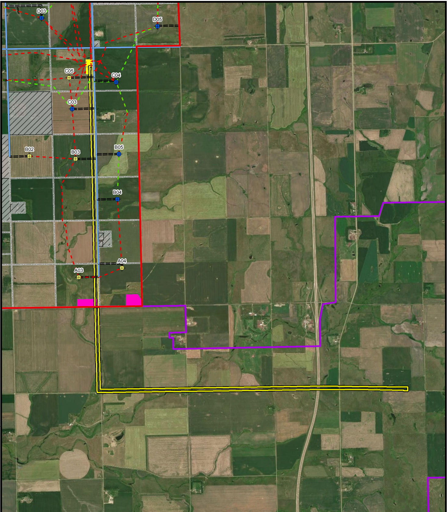
FIGURE 4: TRANSMISSION FACILITY LAYOUT REV. 12/10/18 DAKOTA RANGE III WIND ENERGY FACILITY & TRANSMISSION LINE SDPUC APPLICATION BURNS McDONNELL SM
