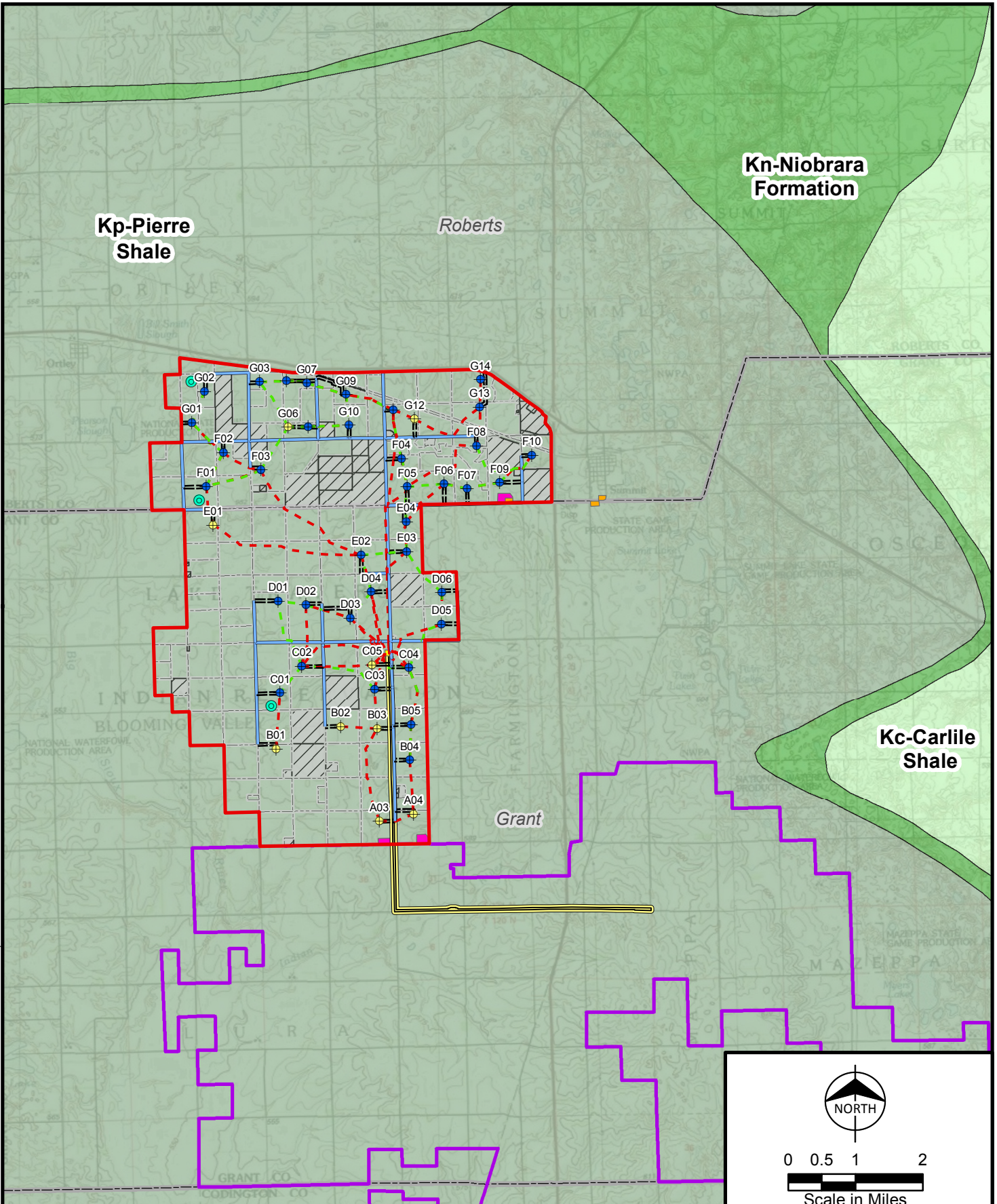
FIGURE 10: BEDROCK GEOLOGY REV.12/10/18 DAKOTA RANGE III WIND ENERGY FACILITY & TRANSMISSION LINE SDPUC APPLICATION
