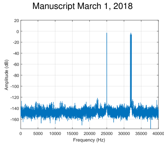
Figure 17: Calculated spectrum of 25 kHz tone and 180 Hz AM modulated over a 32 kHz carrier.
