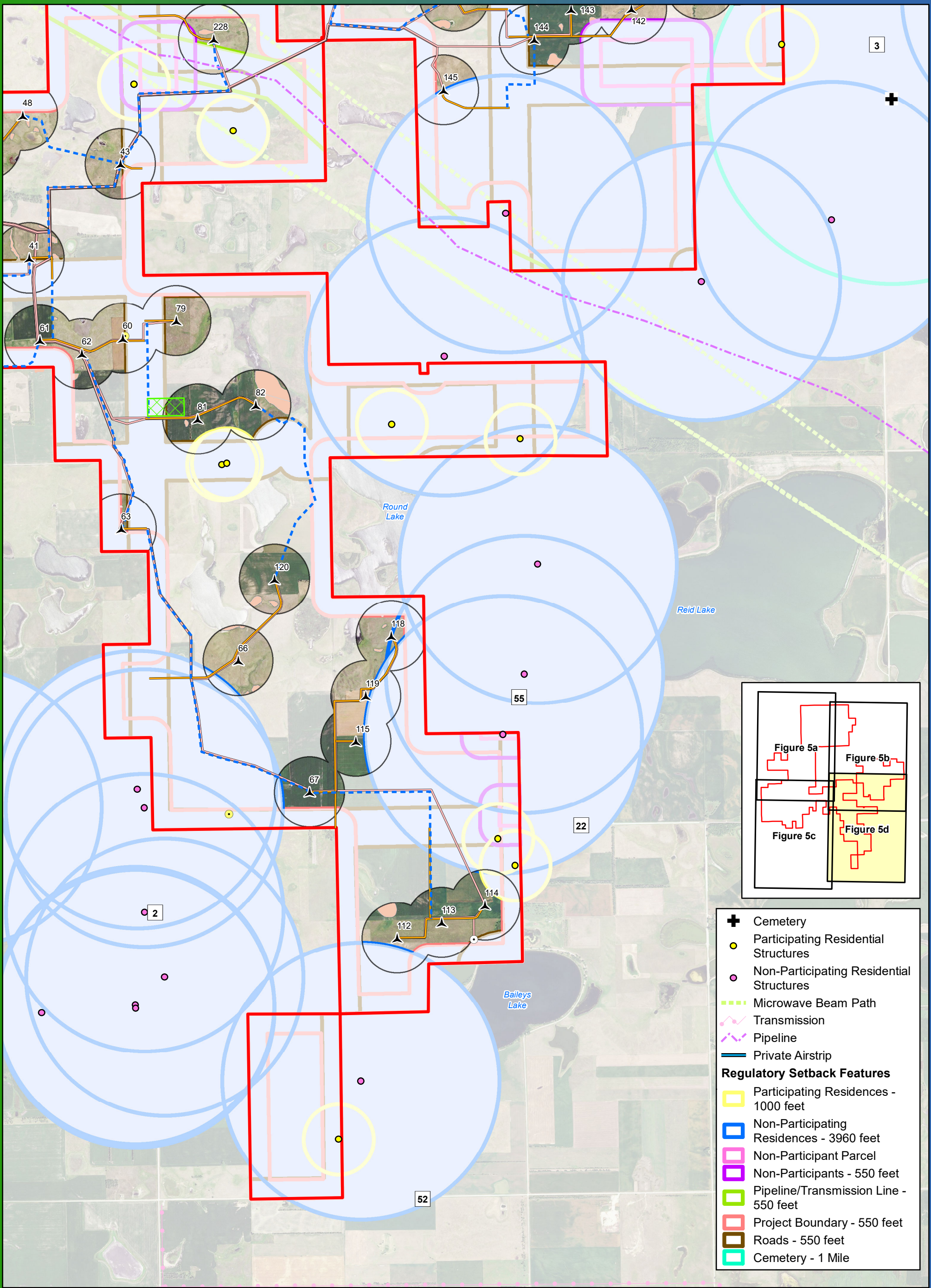
Figure 5d Project Micrositing (Detailed)
