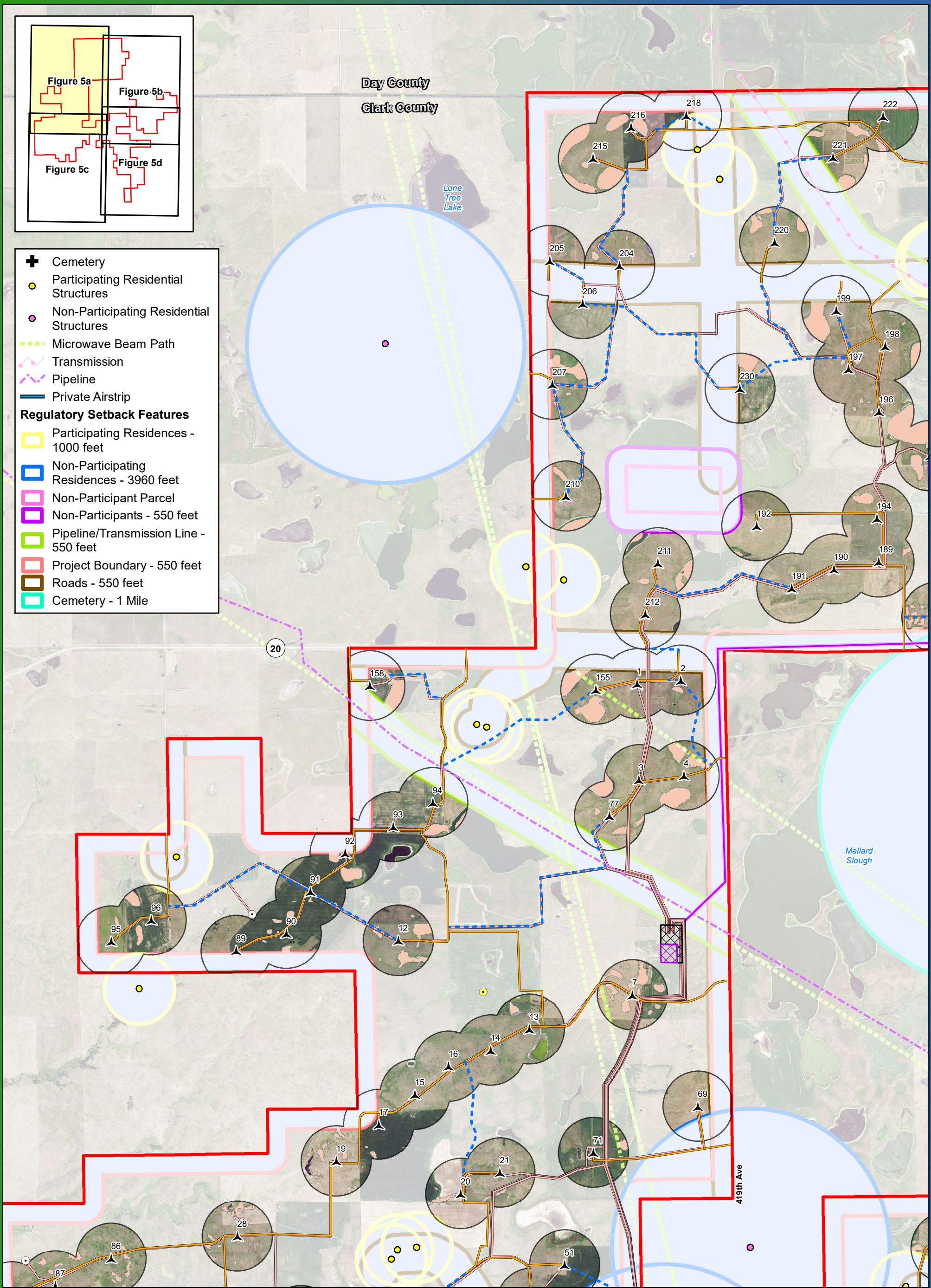
Figure 5a Project Micrositing (Detailed)
