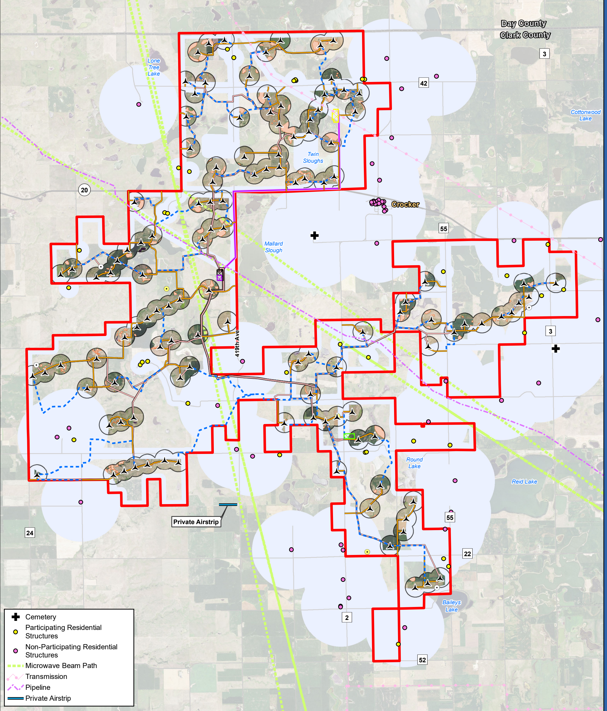
Figure 5 Project Micrositing Crocker Wind Farm Clark County, SD 45.079602, -97.845696
