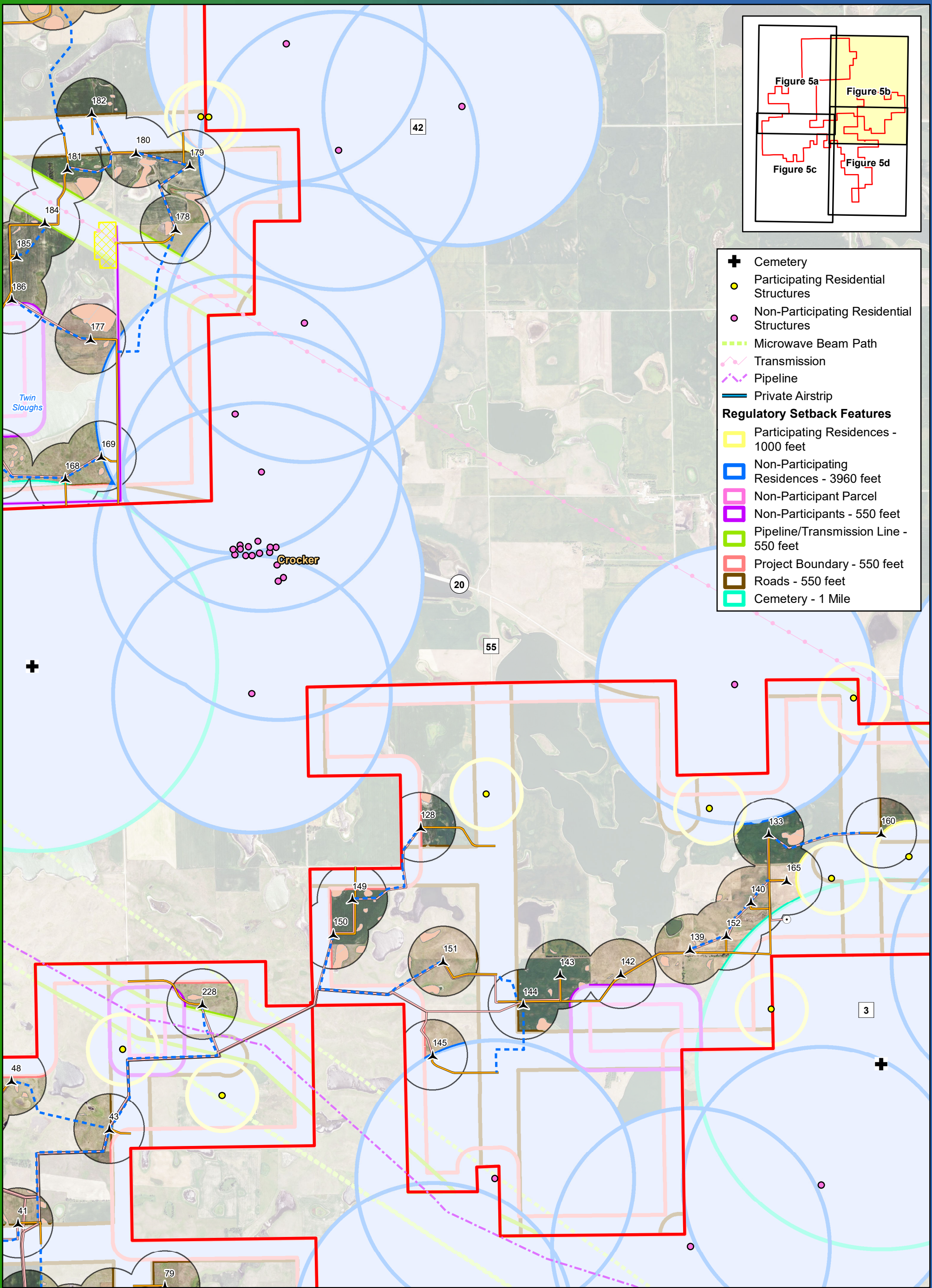
Figure 5b Project Micrositing (Detailed)
