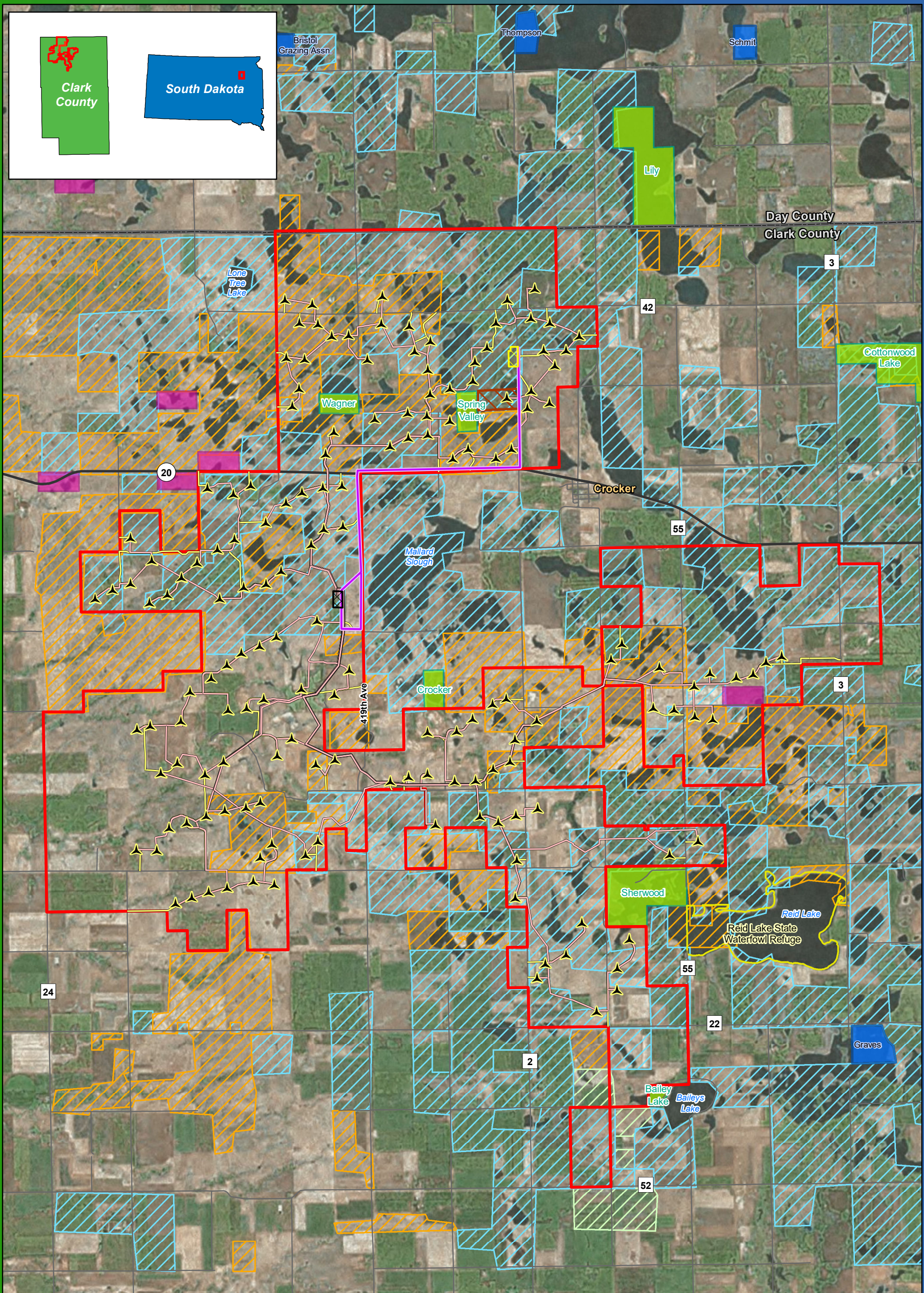
Figure 7c Public Lands and Recreation GE 2.5-116 Crocker Wind Farm Clark County, SD 45.079602, -97.845696
