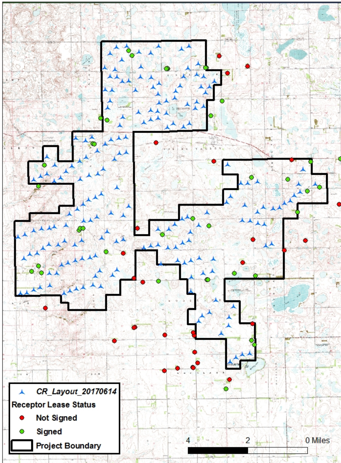
Figure 1 - Crocker Wind Farm layout with receptors
